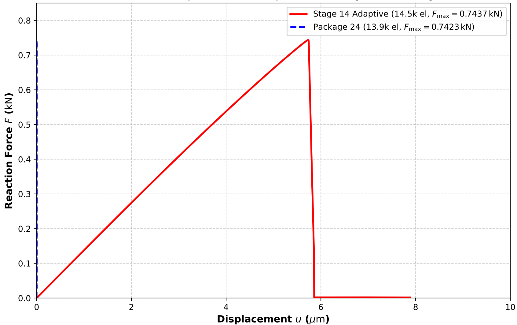
Mode-I Force-Displacement Response: Package 24 vs Stage 14
