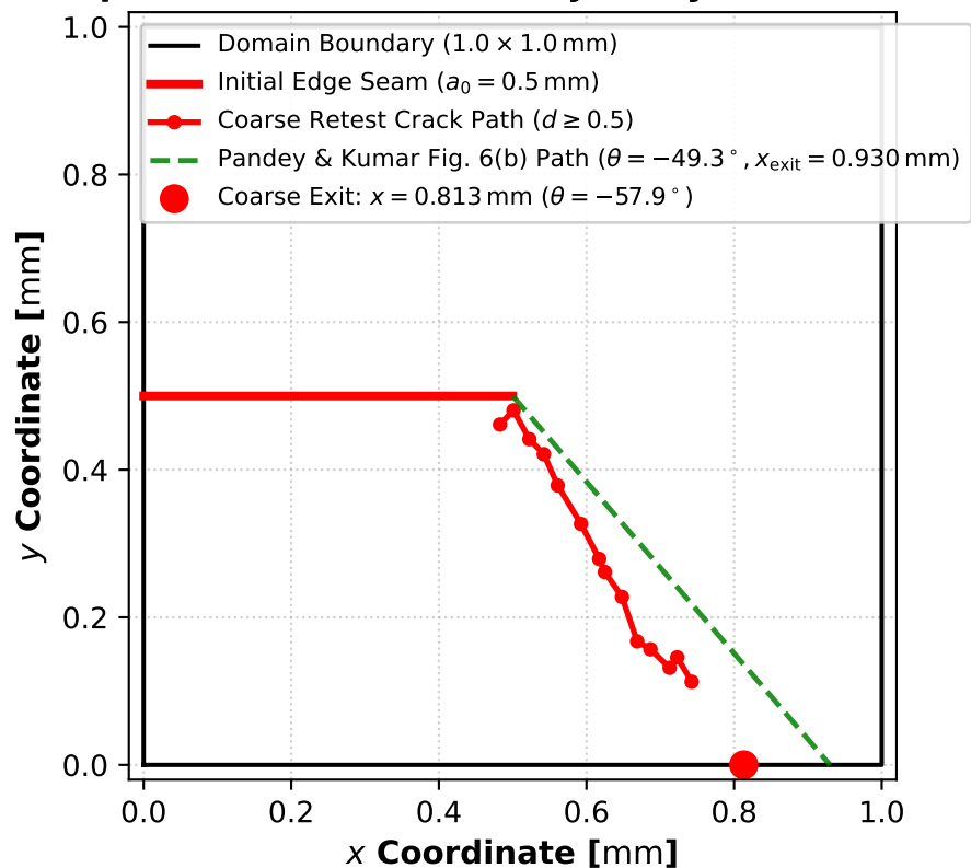
(c) Computed Mode-II Crack Trajectory vs Literature Path
