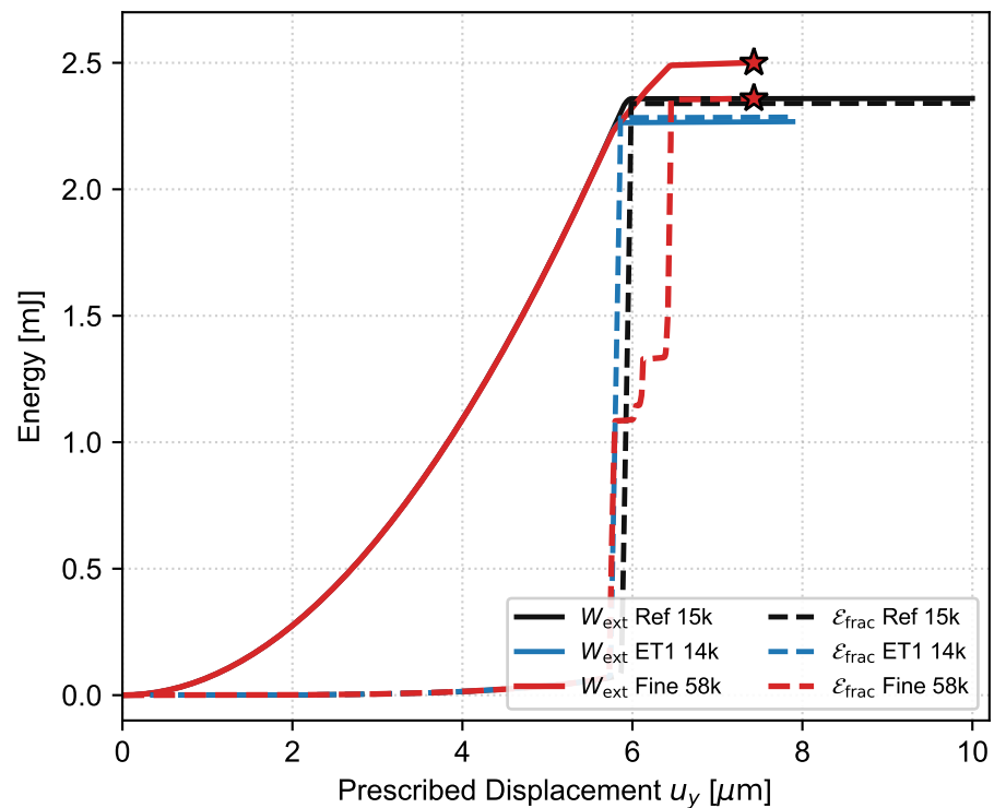
(b) External Work W_{\text{ext}} & Fracture Energy \mathcal{E}_{\text{frac}}
