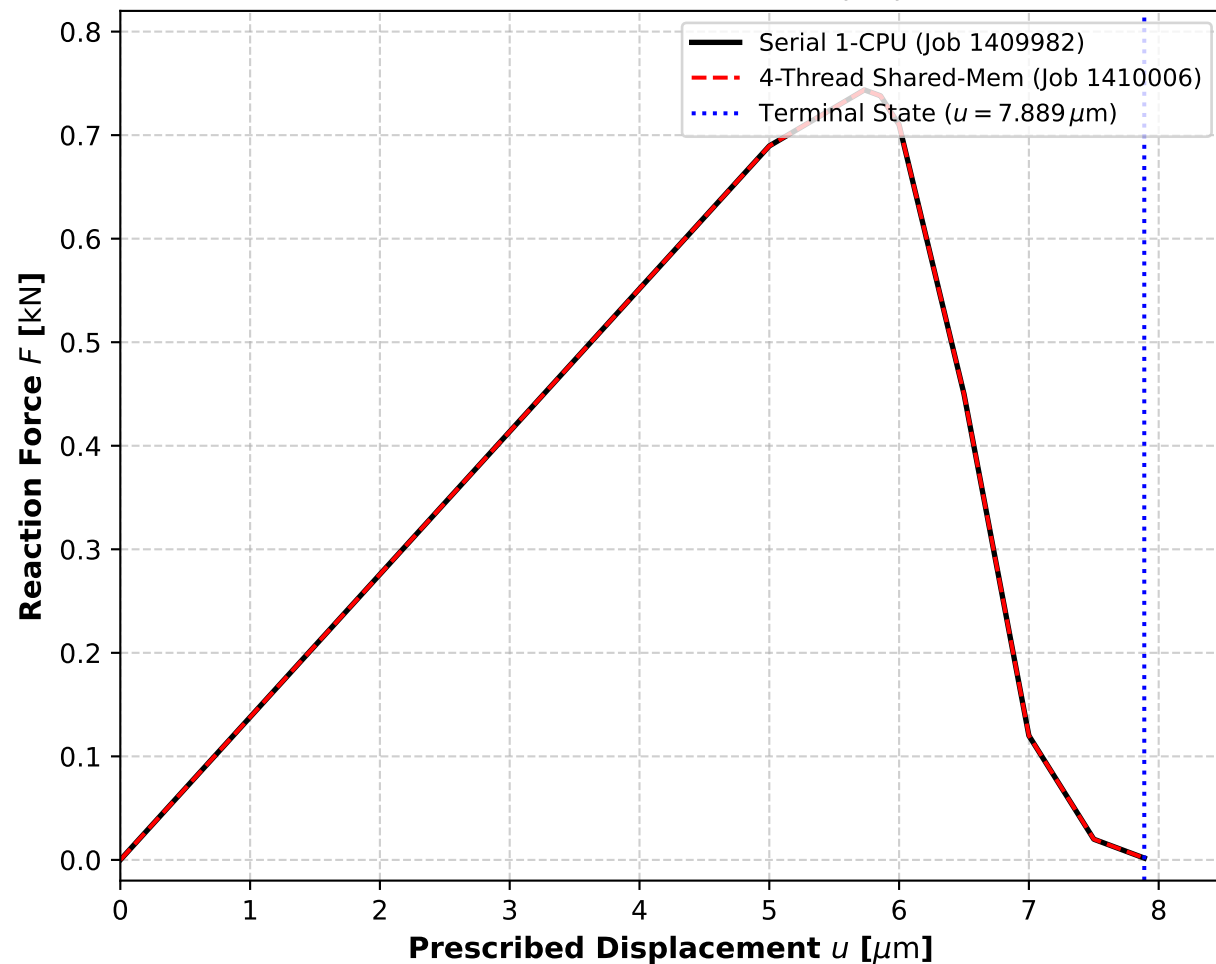
(a) Mechanical Response Parity ( |\Delta F| = 0.000 kN)
