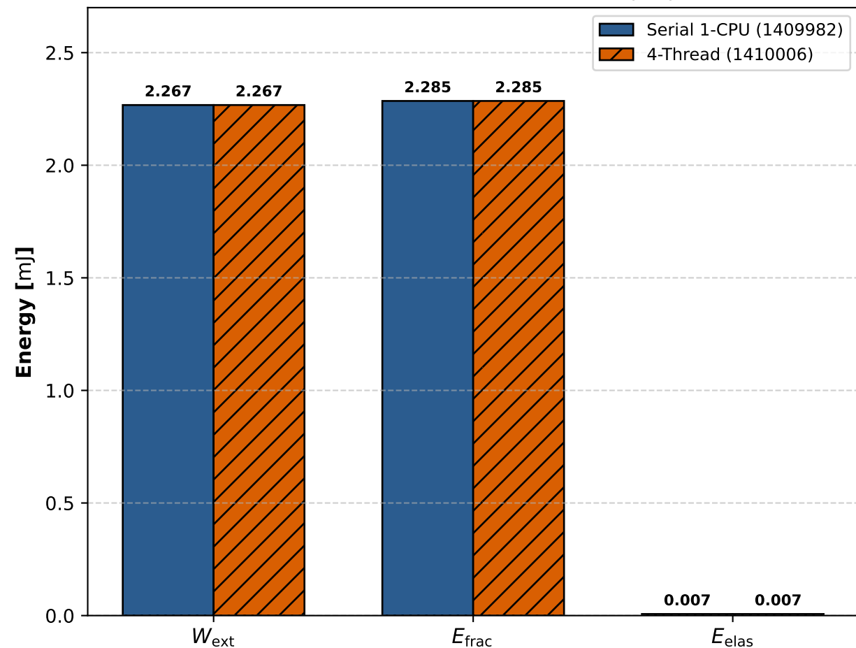
(b) Terminal Energy Functional Parity ( |\Delta E| = 0.000 mJ)
