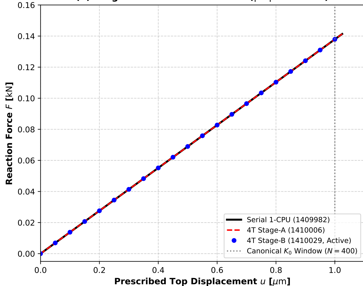
(a) Stage-B Elastic Determinism ( |\Delta F| = 0.000 kN)
