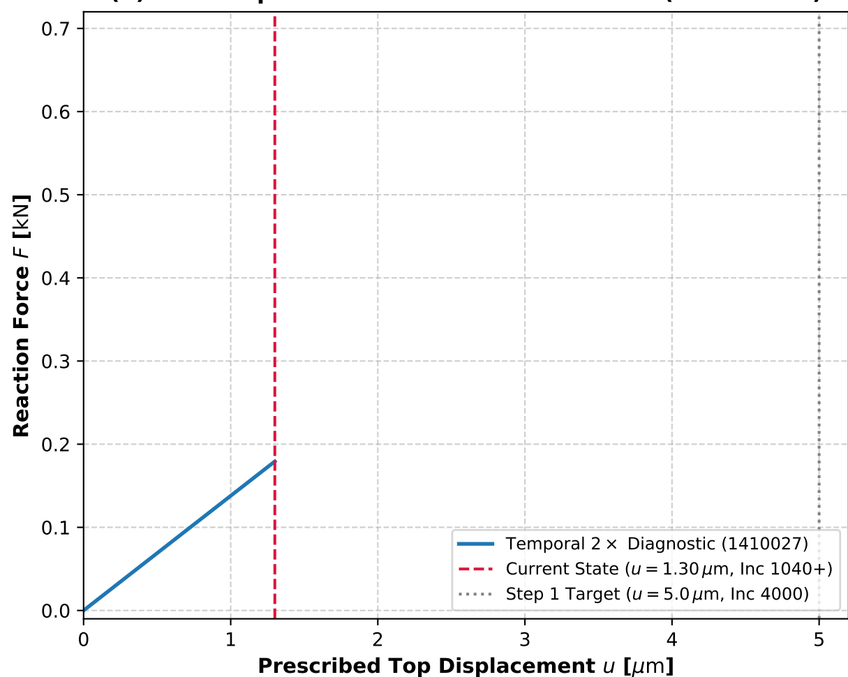
(b) 2 \times Temporal Refinement Advancement (0 Cutbacks)
