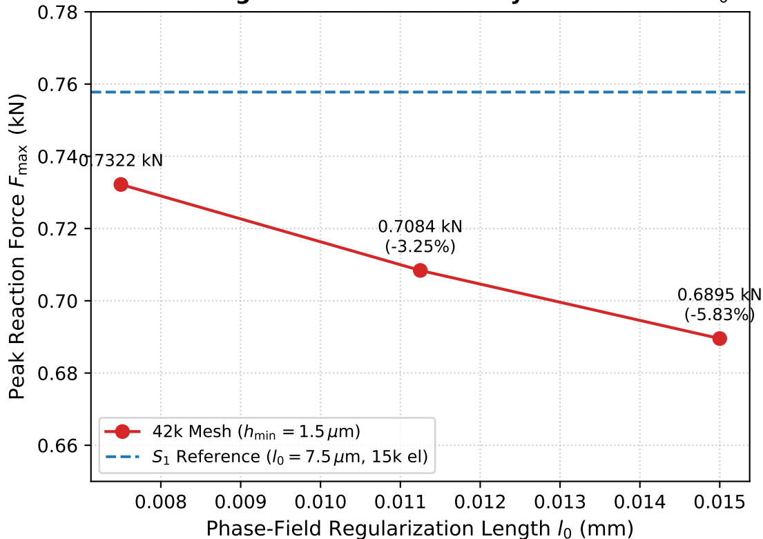
Mode-I Regularization Sensitivity: Peak Load vs l_0
