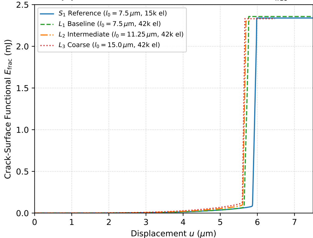
(b) Phase-Field Crack-Surface Functional E_{\text{frac}}
