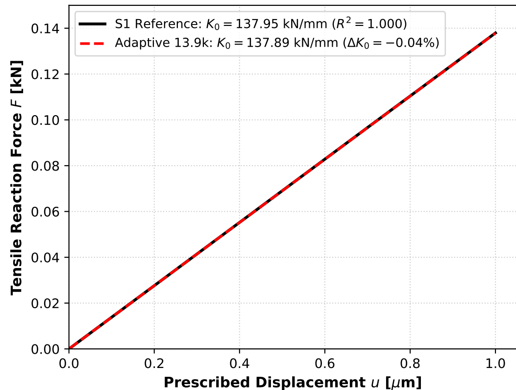
(b) Initial Elastic Compliance ( u \leq 1.0 \mu\text{m} )
