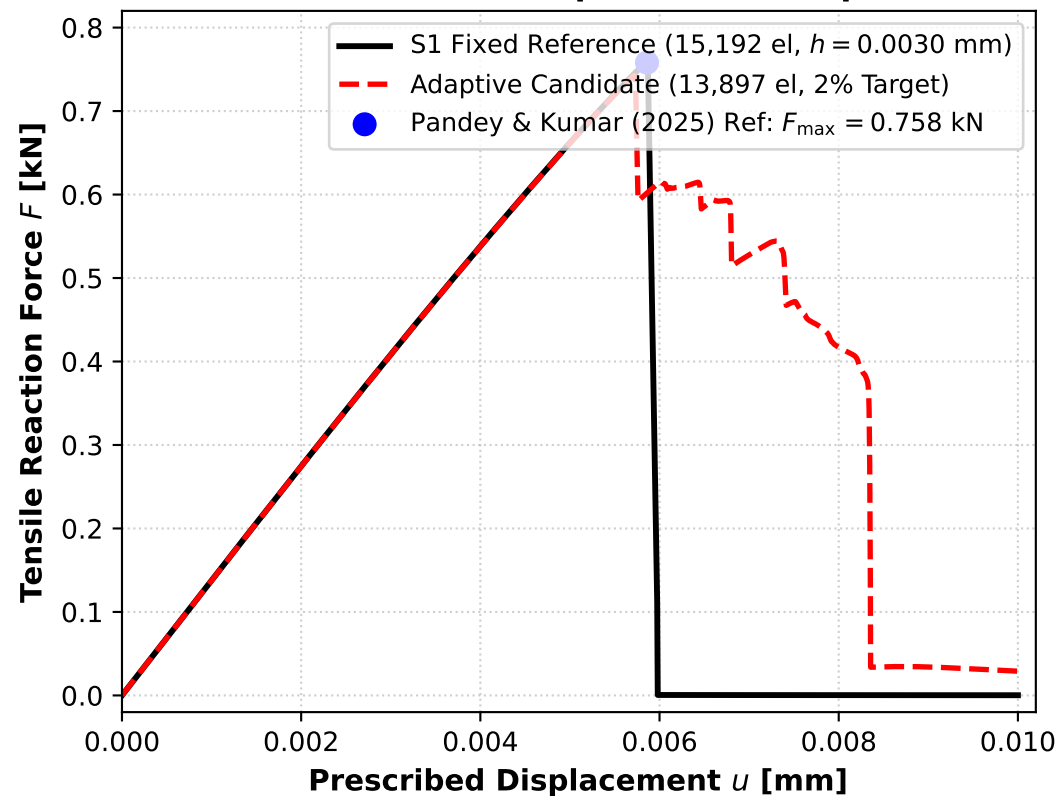
(a) Mode-I Force-Displacement Response
