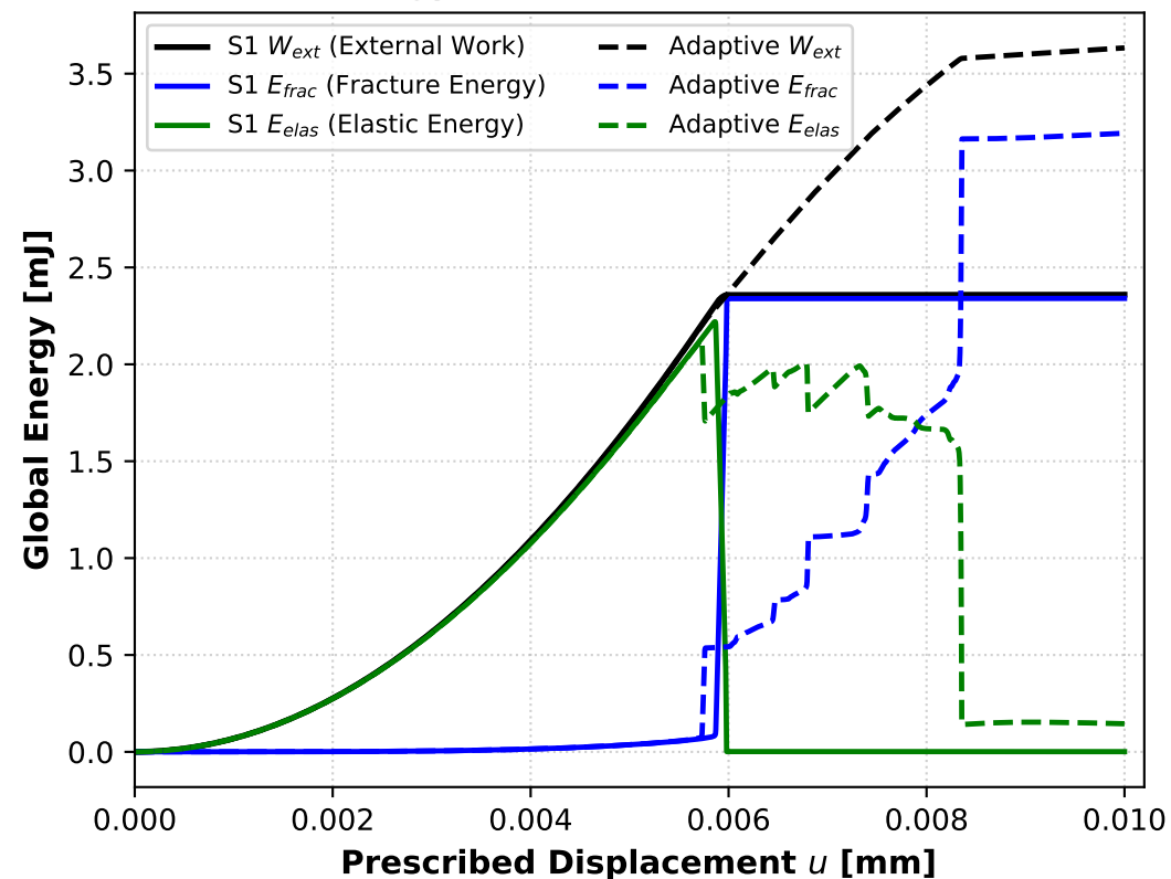
(c) Global Energy Evolution ( 1 \text{ kN} \cdot \text{mm} = 1.0 \text{ J} = 1000 \text{ mJ} )
