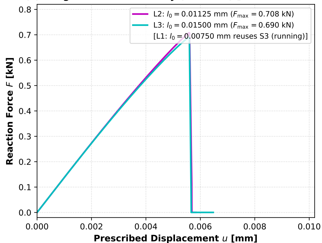
(c) Length-Scale Sensitivity (L2 → L3) [Material Effect]
