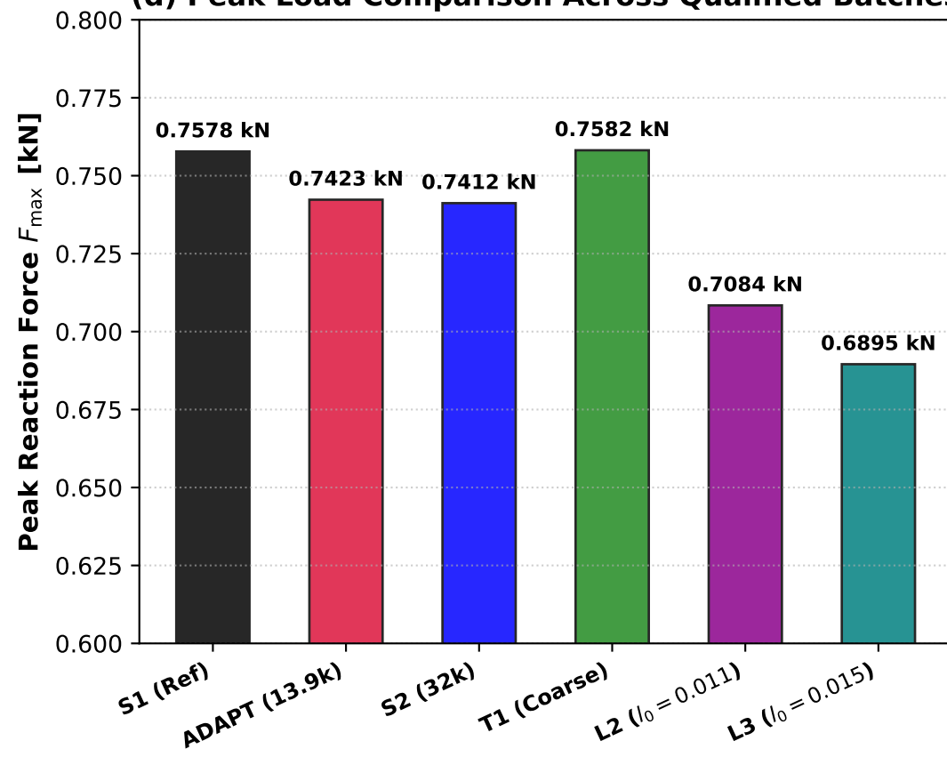
(d) Peak Load Comparison Across Qualified Batches
