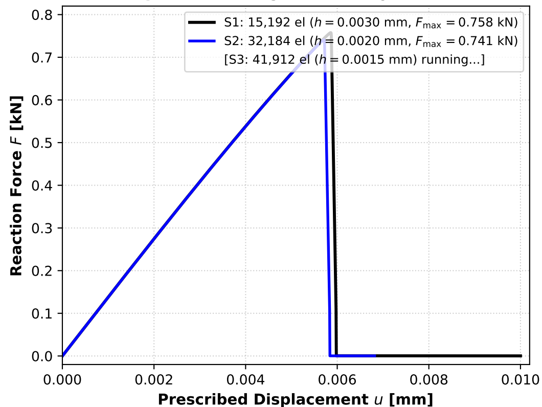
(a) Spatial Convergence Family (S1 → S2)
