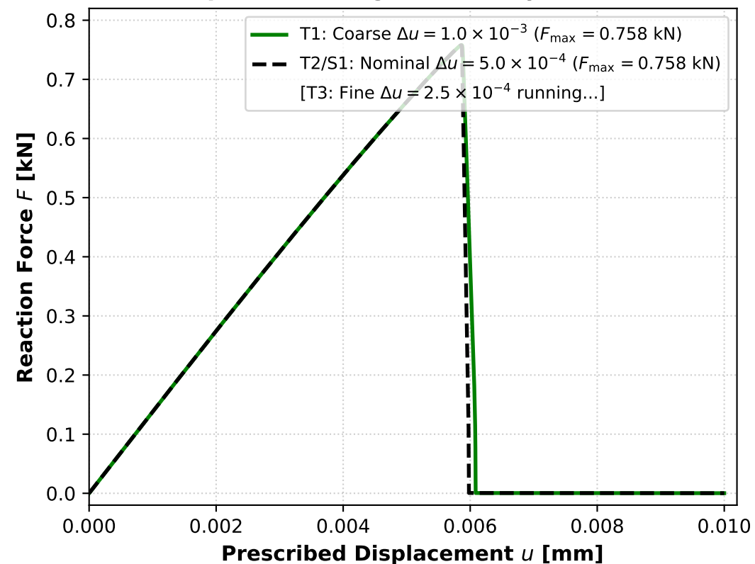
(b) Temporal Convergence Family (T1 → T2/S1)
