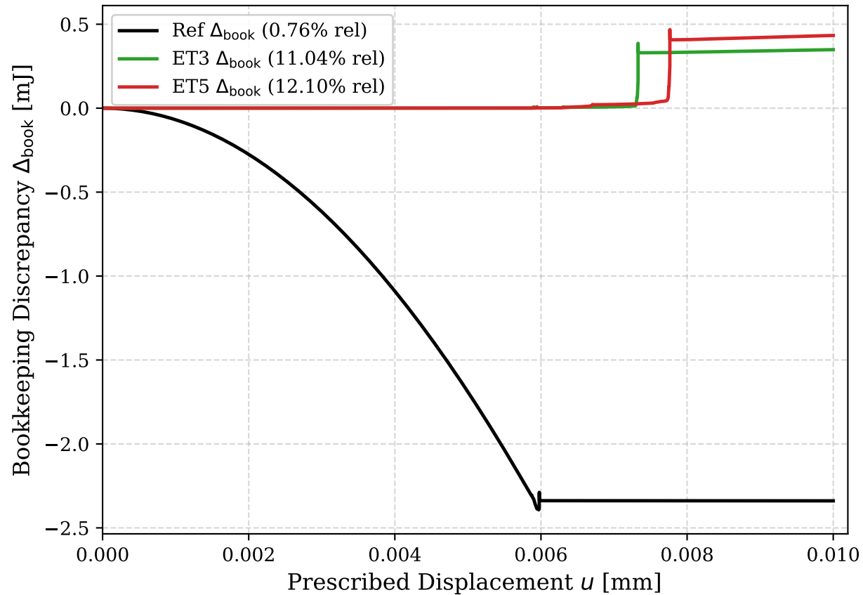
Energy Balance Discrepancy ( \Delta_{\text{book}} = W_{\text{ext}} - \mathcal{E}_{\text{model}} )
