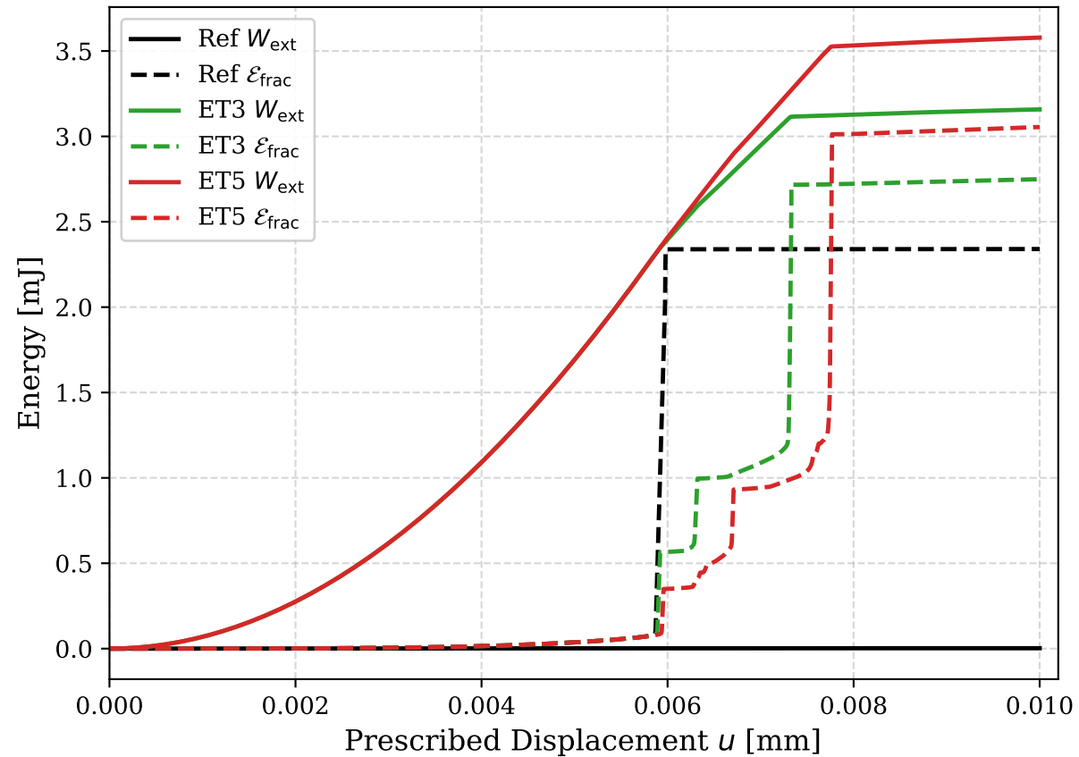
External Work & Implemented Fracture Energy
