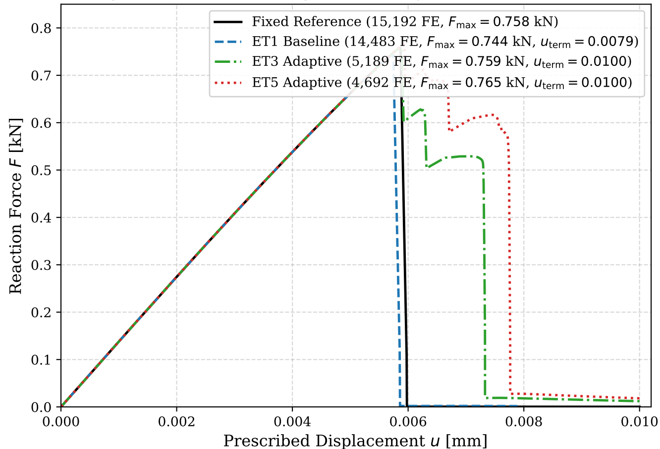
Mode-I Stage-14 Step-2 ErrorTarget Sensitivity: Force-Displacement Response
