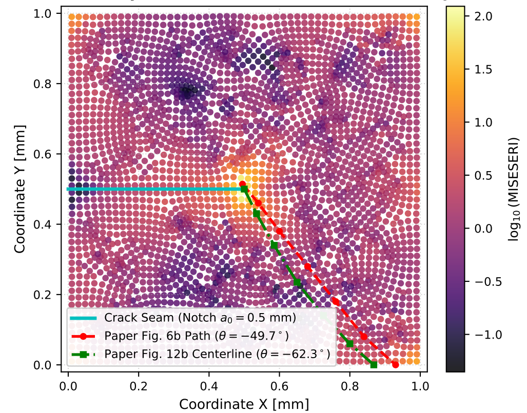
(b) Coarse Pre-Analysis ( h = 0.02 mm, 2,960 CPE4) vs. Paper Paths
