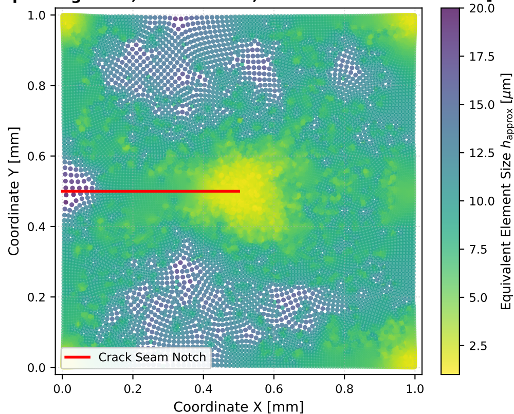
(c) Native Adaptive Discretization (errorTarget=2.0, 21,496 elements) [Paper target: 19,963 elements; relative difference: +7.7%]
