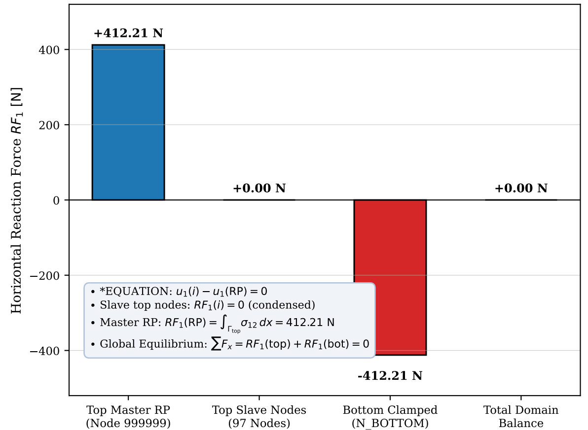
(b) Global Boundary Equilibrium &amp; *EQUATION MPC Verification
