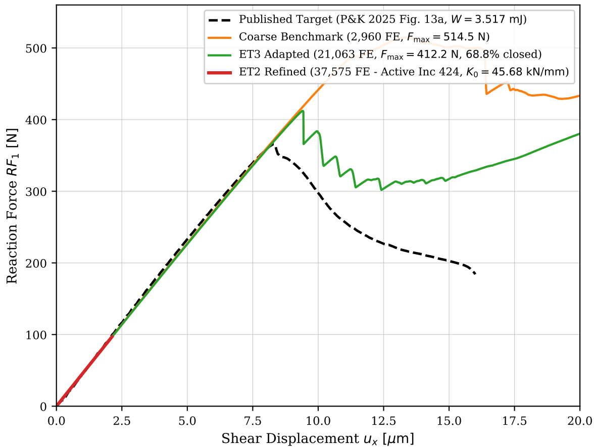
(c) Multi-Discretization Mechanical Comparison &amp; Active ET2 Tracking
