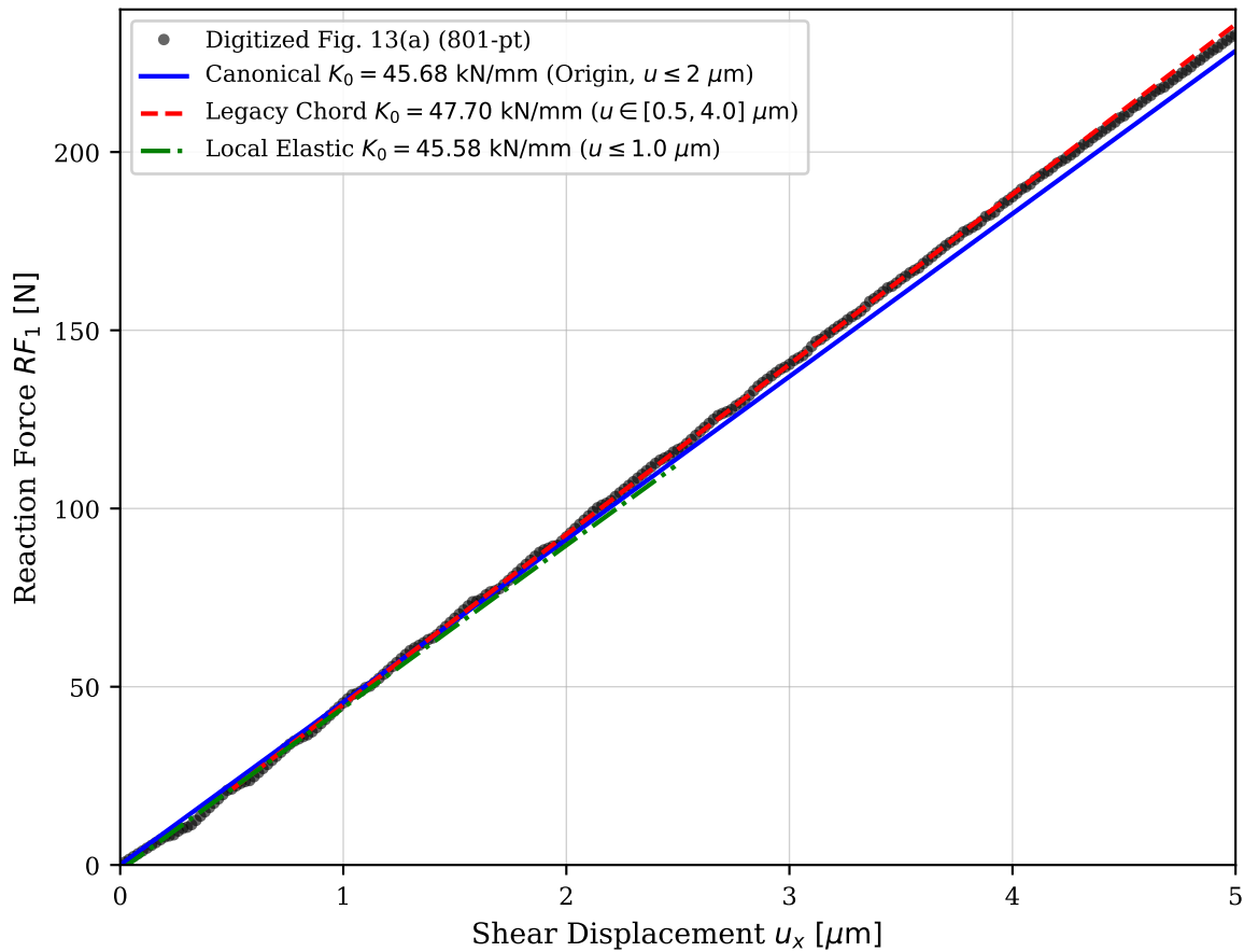
(a) Reference Initial Stiffness Reconciliation (Pandey &amp; Kumar Fig. 13a)
