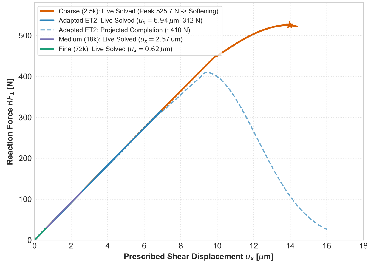
(c) Live Progressive Loading & Post-Peak Softening Curves
