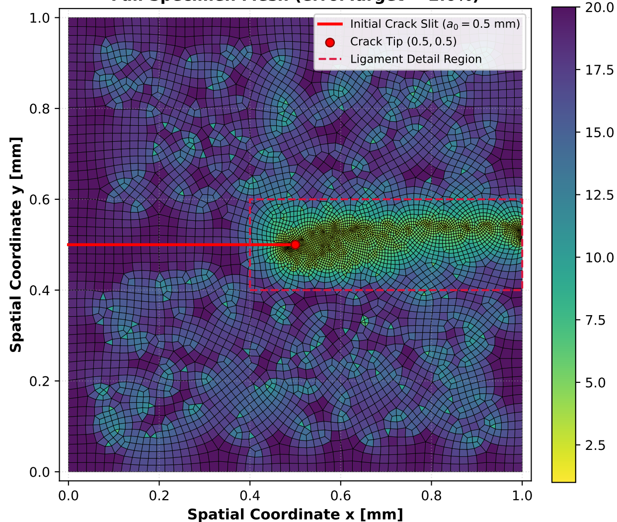
Full Specimen Mesh (errorTarget = 2.0%)
