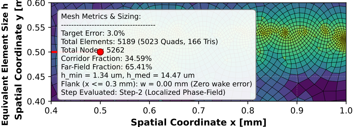
Ligament Detail: x in [0.4, 1.0], y in [0.4, 0.6] mm
