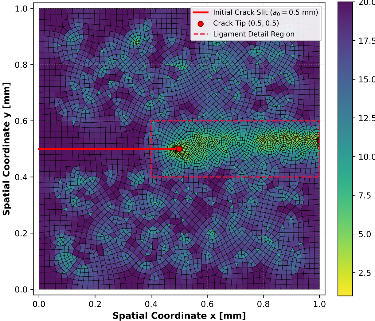
Full Specimen Mesh (errorTarget = 5.0%)
