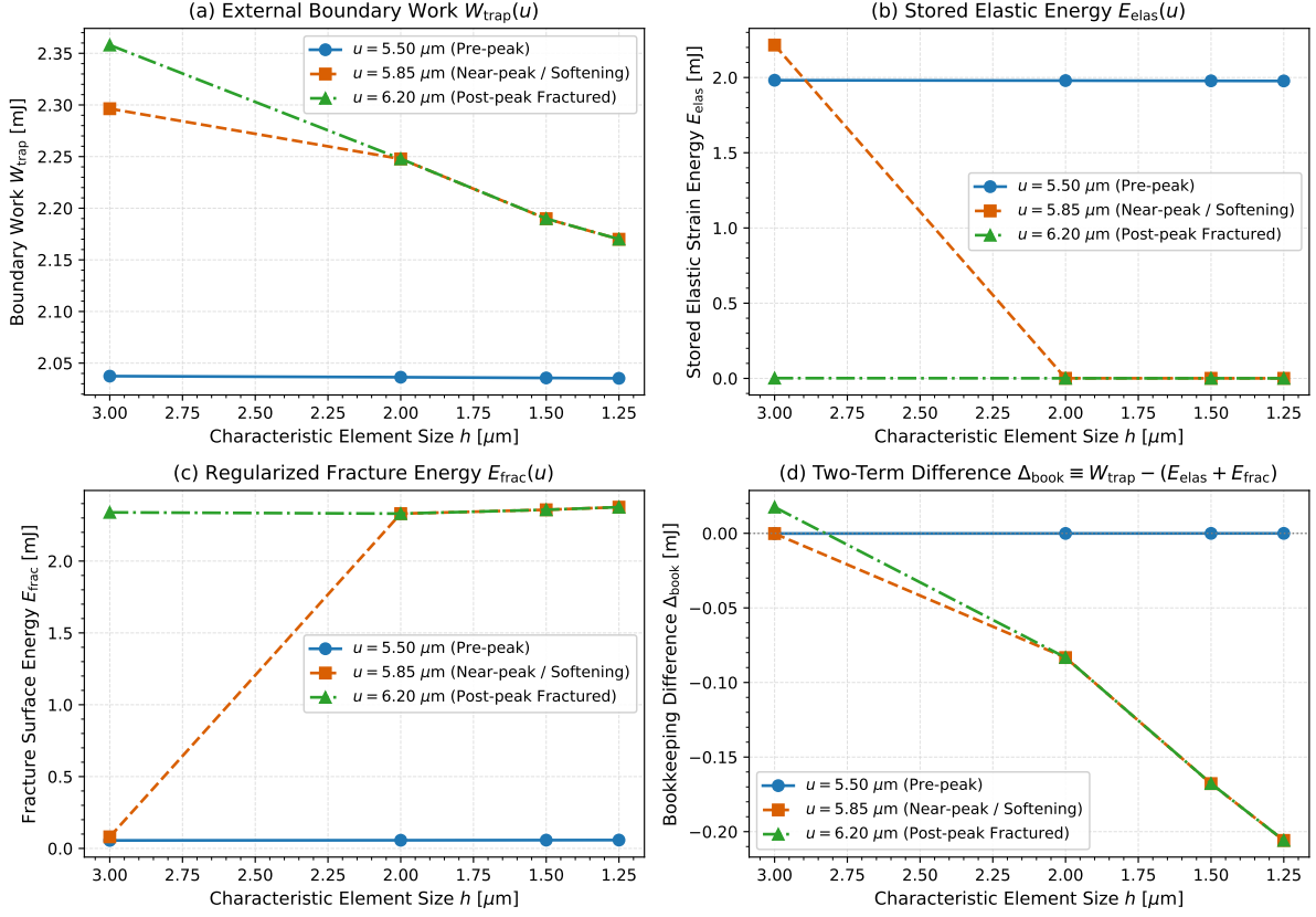
Figure 30: Spatial discretization convergence of global energy components across meshes S_1 – S_4 at matched displacements u = 5.50, 5.85, 6.20 \mu\text{m} : (a) boundary work W_{\text{trap}} ; (b) stored elastic strain energy E_{\text{elas}} ; (c) regularized fracture surface energy E_{\text{frac}} ; (d) two-term bookkeeping difference \Delta_{\text{book}} . GLOBAL_ENERGY_IDENTITY -- NOT_YET_CLOSED.
