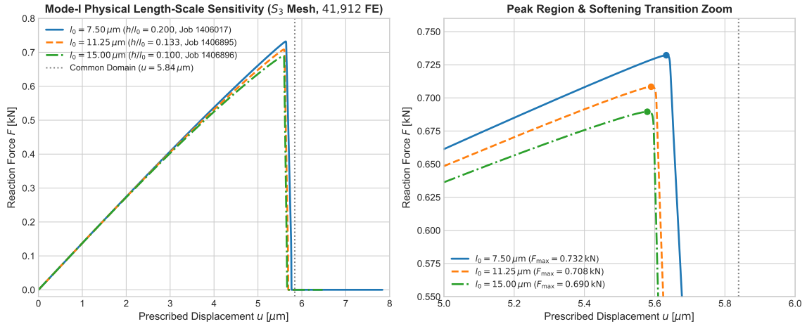
Figure 19: Mode-I clean single-variable length-scale ( l_0 ) sensitivity on fixed structured S_3 mesh (41,912 FE): (a) global F - u response highlighting common comparison domain u \in [0, 5.839] \mu\text{m} ; (b) peak-neighborhood zoom illustrating monotonic load reduction and earlier peak displacement with increasing l_0 .
