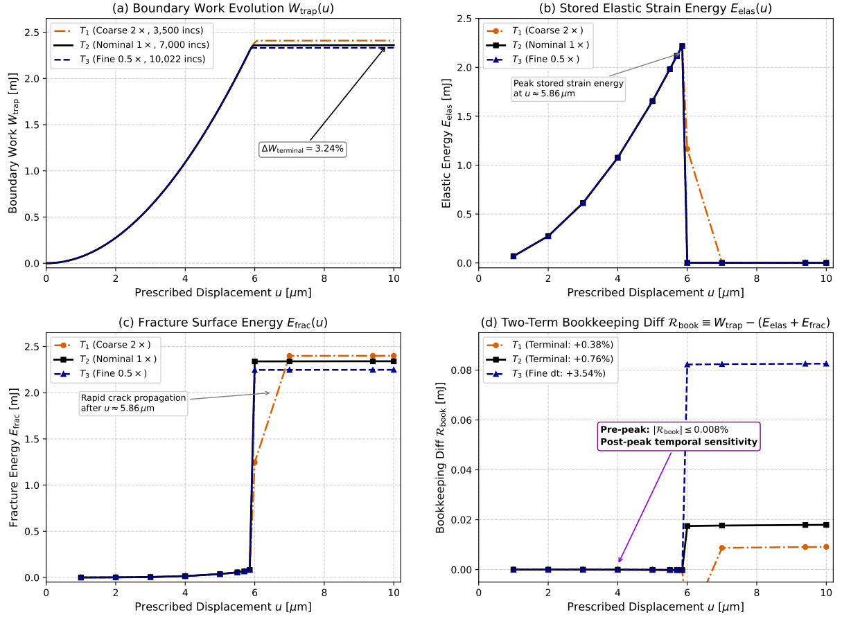
Figure 29: Temporal discretization scaling of global energy components across schedules T_1 ( 2 \times ), T_2 ( 1 \times ), and T_3 ( 0.5 \times , Job 1406317) on fixed S_1 mesh: (a) boundary work W_{\text{trap}}(u) ; (b) stored elastic energy E_{\text{elas}}(u) ; (c) fracture surface energy E_{\text{frac}}(u) ; (d) two-term bookkeeping difference \Delta_{\text{book}}(u) .
