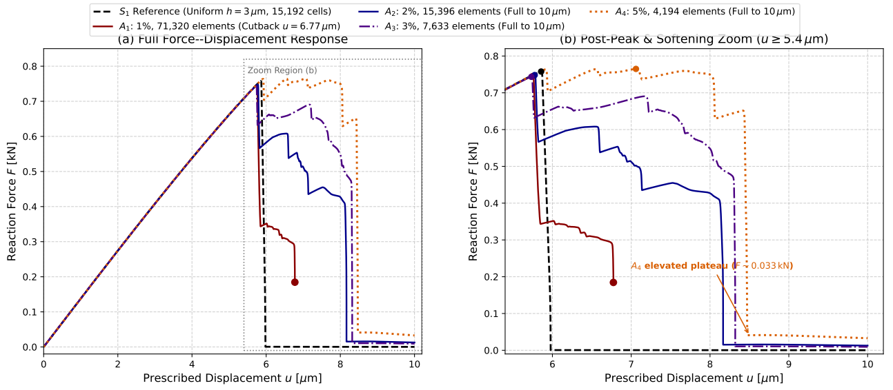
Figure 22: Force–displacement response of the canonical uniform reference S_1 and native adaptive meshes A_1 – A_4 : (a) full response over u \in [0, 10] \mu\text{m} ; (b) post-peak zoom over u \in [5.4, 10] \mu\text{m} . Production adaptive meshes contain 71,320, 15,396, 7,633, and 4,194 underlying finite elements for errorTarget values of 1%, 2%, 3%, and 5%, respectively. A_1 terminates at u = 6.77 \mu\text{m} , whereas A_2 – A_4 reach 10 \mu\text{m} .
