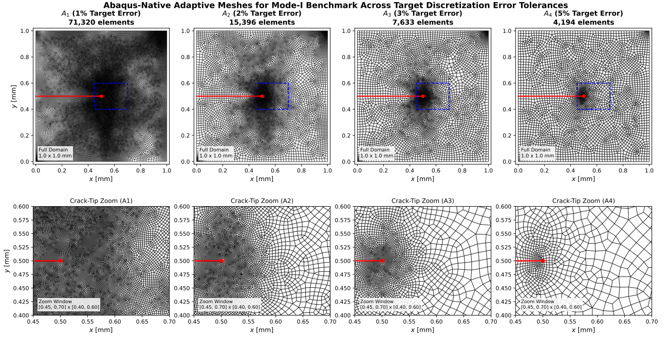
Figure 21: Abaqus-native adaptive meshes generated for the Mode-I benchmark using errorTarget values of (a) 1%, (b) 2%, (c) 3%, and (d) 5%. The corresponding production meshes contain 71,320, 15,396, 7,633, and 4,194 underlying finite elements, respectively. Full-domain views and identical crack-tip zooms illustrate how relaxing the target error changes the spatial refinement distribution.
