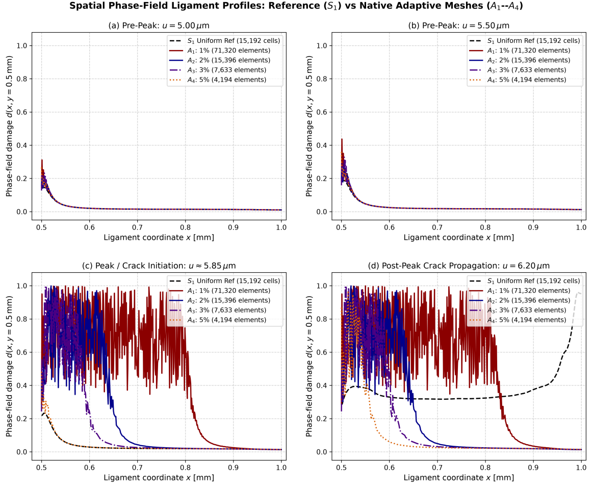
Figure 25: Spatial phase-field ligament profiles d(x, y = 0.5 \text{ mm}) comparing canonical reference S_1 against native adaptive meshes A_1 – A_4 across matched displacement levels.
