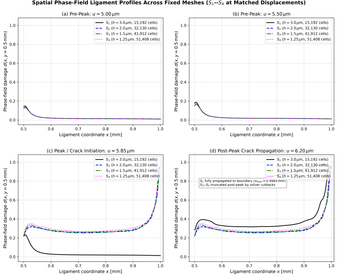
Figure 24: Spatial phase-field ligament profiles d(x, y = 0.5 \text{ mm}) for fixed meshes S_1 – S_4 across matched displacement levels, showing x-axis coordinates on all panels and annotating full boundary propagation in S_1 at u = 6.20 \mu\text{m} .
