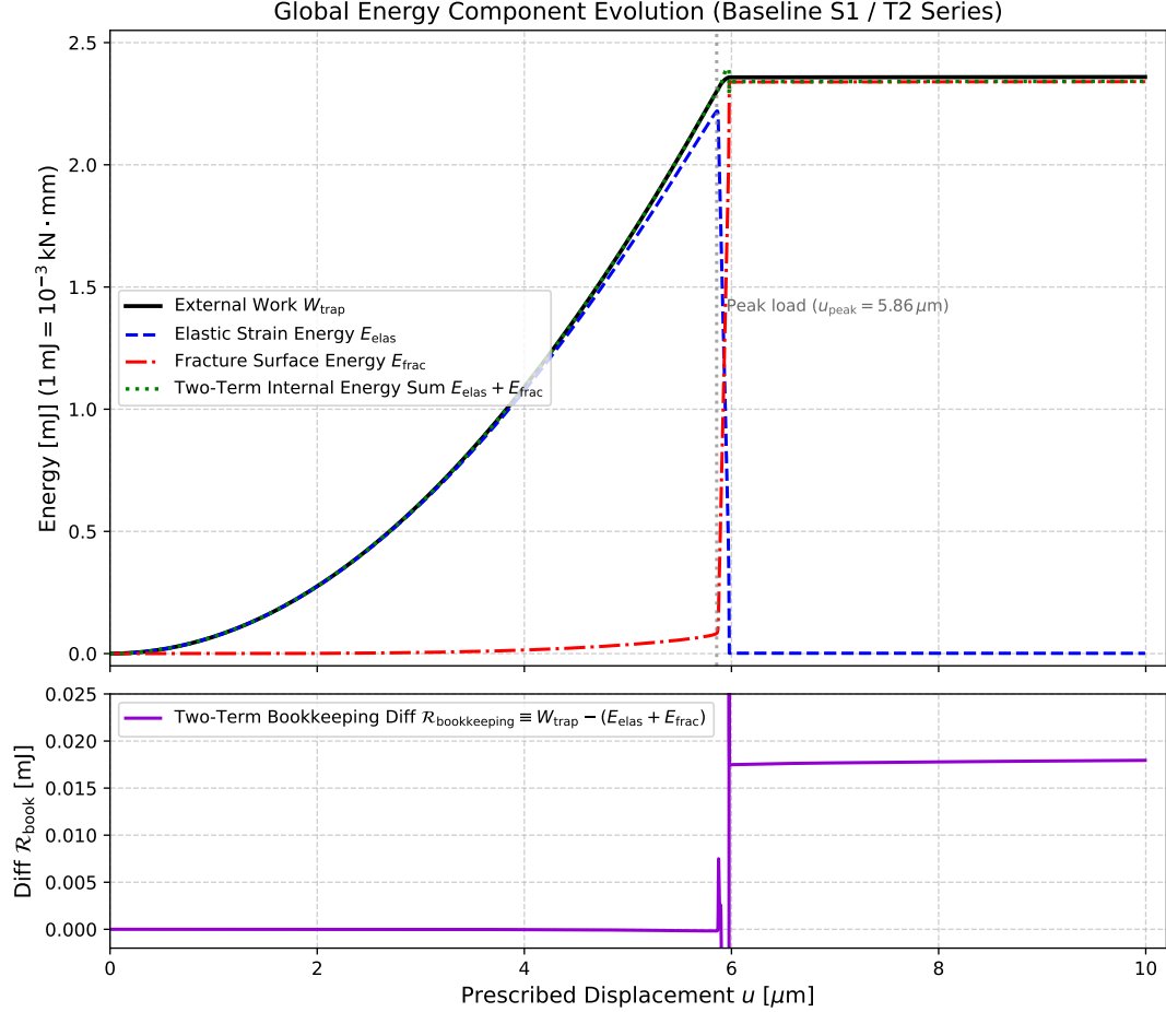
Figure 28: Global energy component evolution for baseline S_1/T_2 (15,192 elements). The two-term bookkeeping difference remains within \pm 0.008\% over pre-peak deformation ( u \leq 5.50 \mu\text{m} ). In the post-peak regime it reaches +0.7607\% for S_1/T_2 . This quantity is an observed endpoint bookkeeping difference: GLOBAL_ENERGY_IDENTITY -- NOT_YET_CLOSED .
