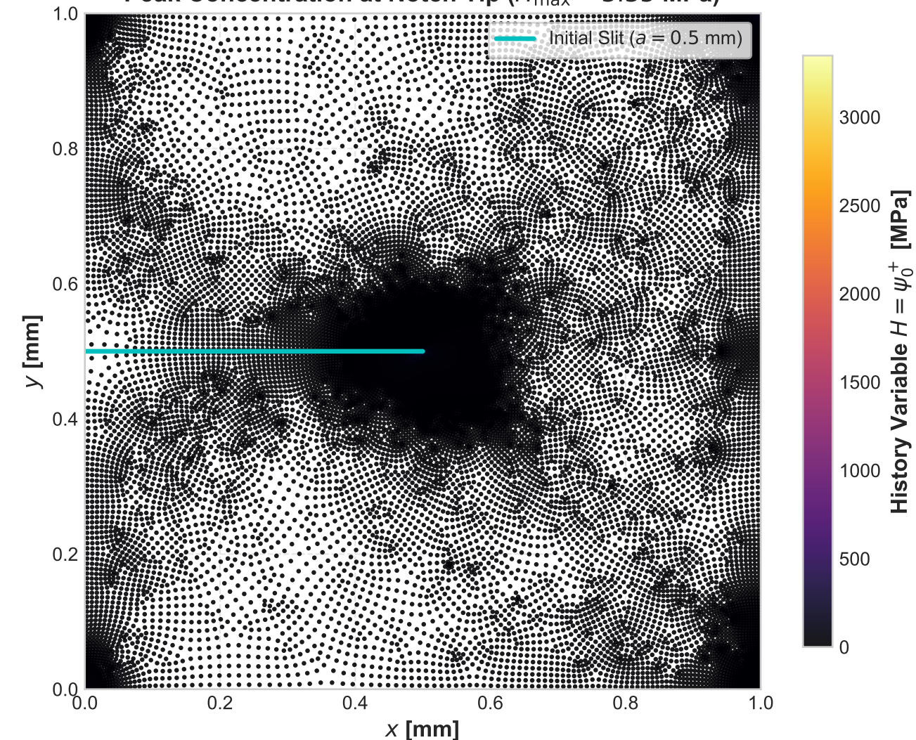
(a) Crack Driving History Variable H(x, y) Peak Concentration at Notch Tip ( H_{\max} = 3.35 MPa)
