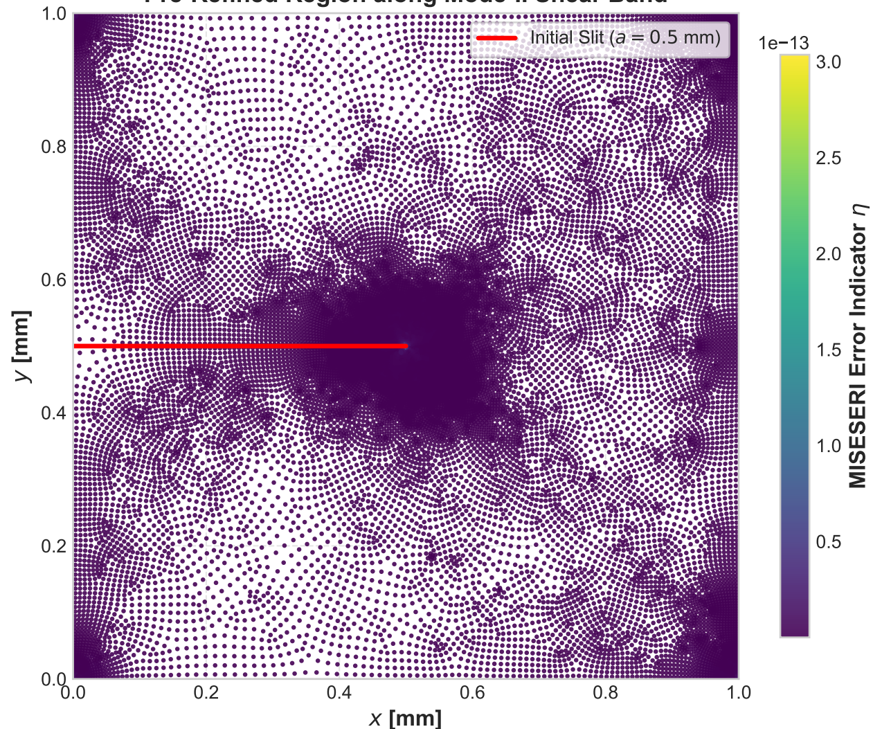
(b) Adapted Mesh MISESERRI Distribution Pre-Refined Region along Mode-II Shear Band
