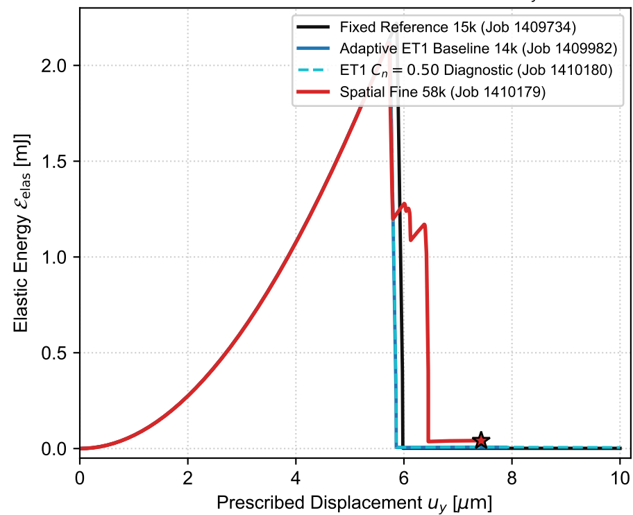
(c) Stored Elastic Strain Energy \mathcal{E}_{\text{elas}}(u_y)
