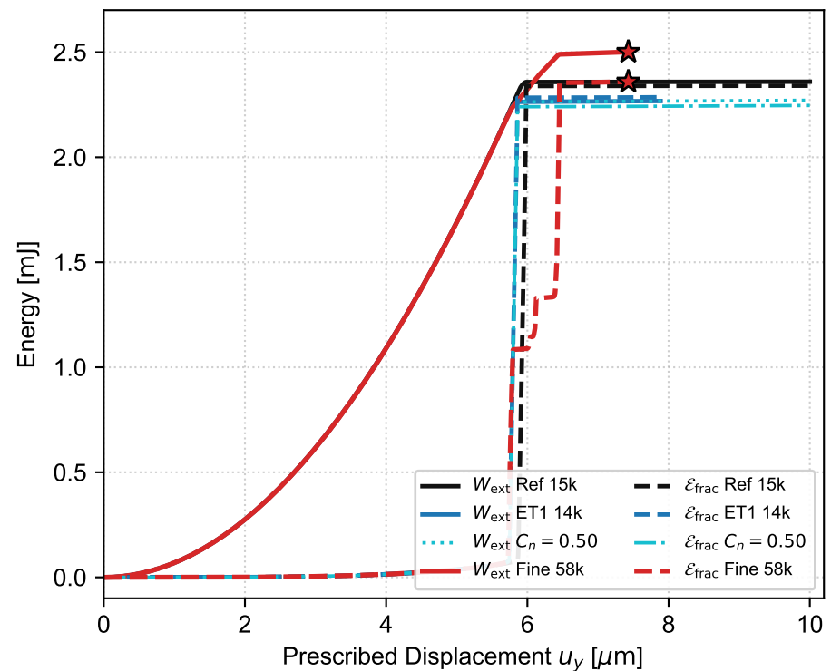
(b) External Work W_{\text{ext}} & Phase-Field Fracture Energy Functional \mathcal{E}_{\text{frac}}
