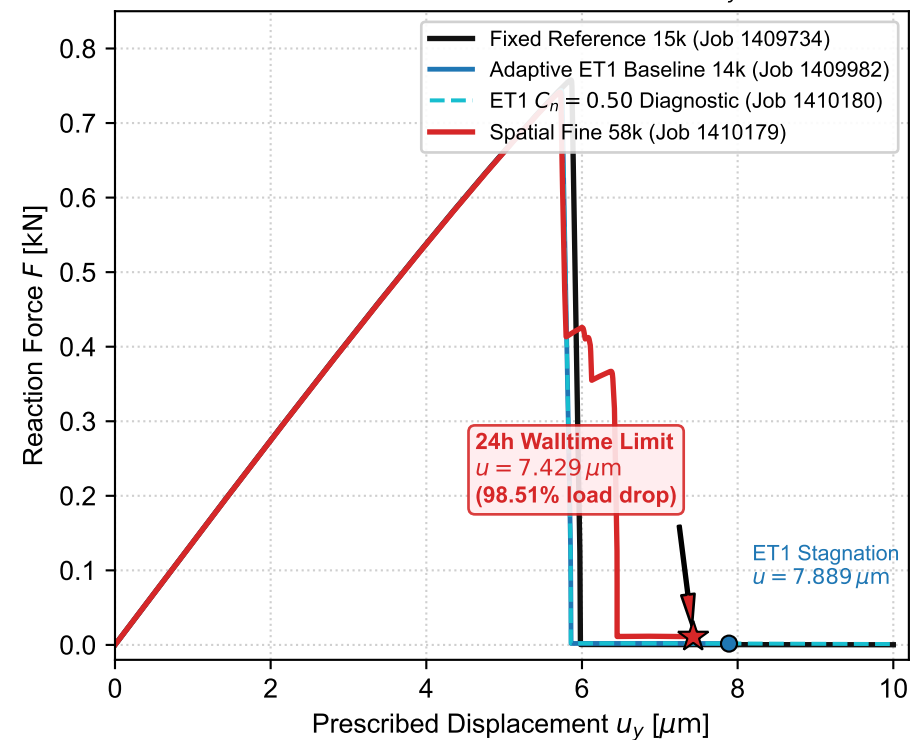
(a) Structural Reaction Force F(u_y)
