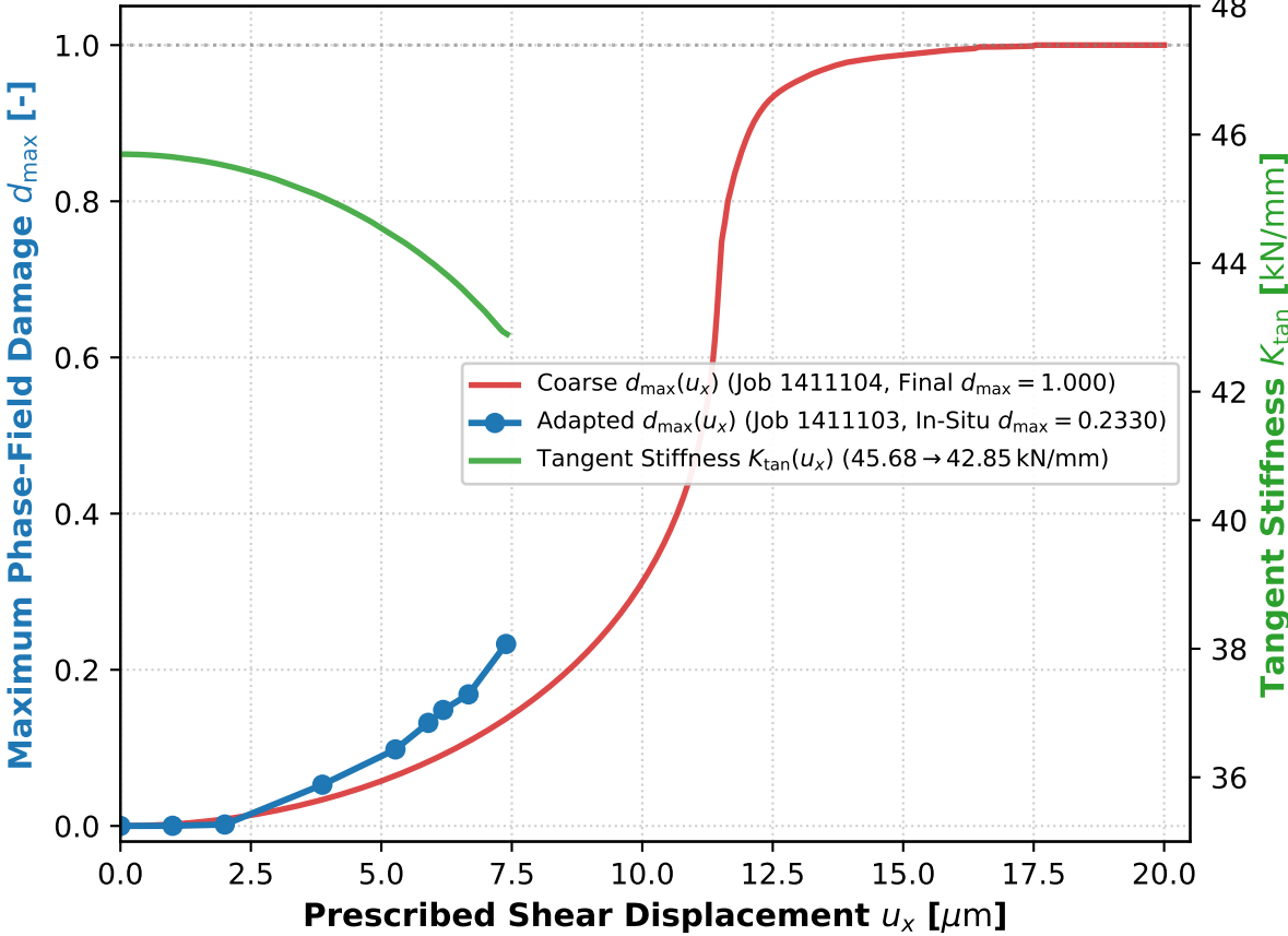
(b) Phase-Field Damage Growth & Stiffness Softening
