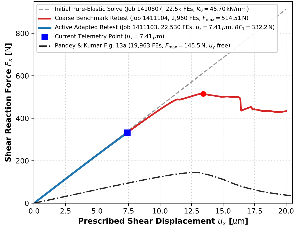
(a) Global Force-Displacement Response & Solver Lineage
