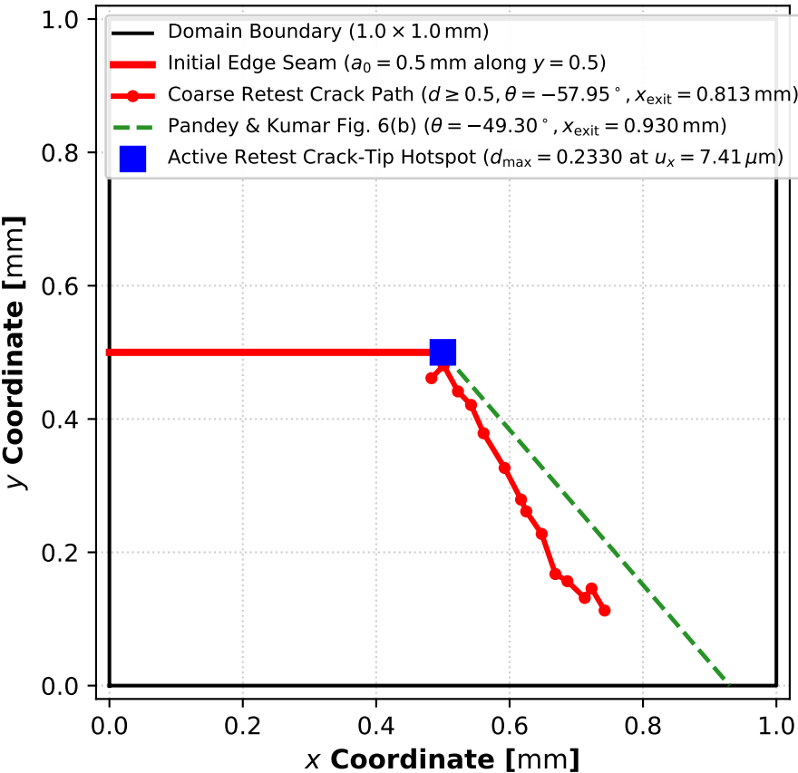
(c) Computed Mode-II Crack Trajectory vs Published Path
