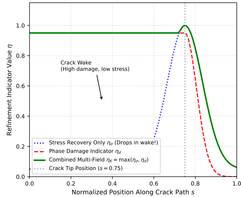
(f) Multi-Field Adaptive Controller: \eta_K = \max(\eta_\sigma, \eta_d)
