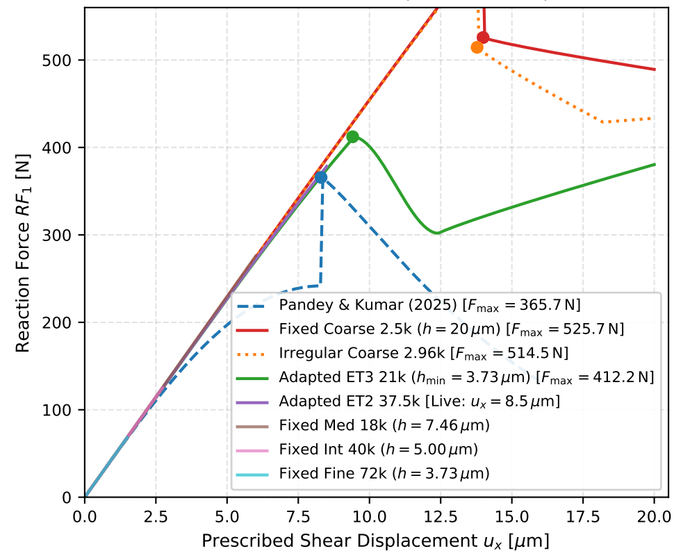
(a) Mode-II Global Load-Displacement Response
