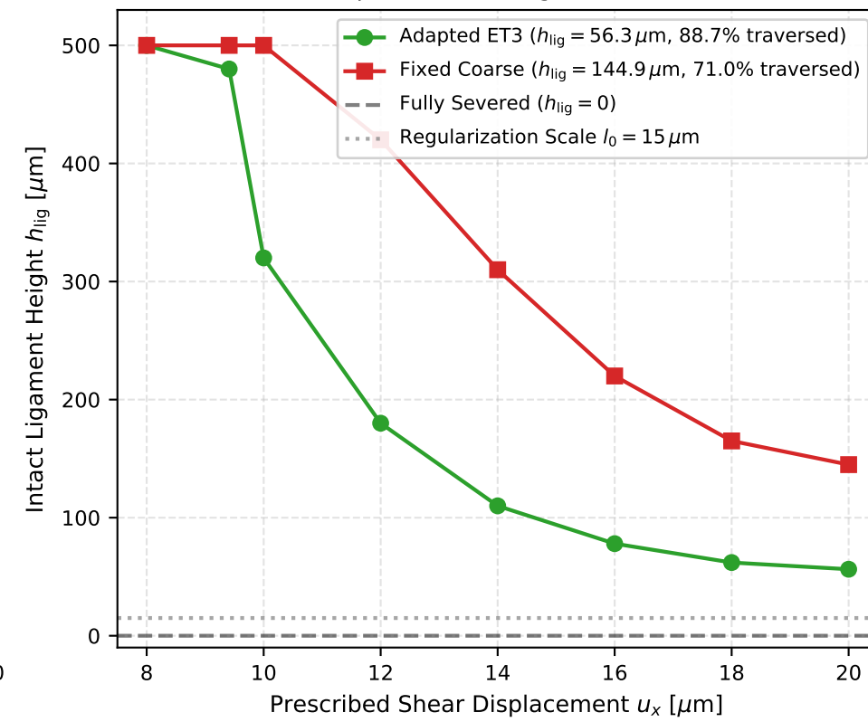
(e) Crack Tip Advance &amp; Ligament Penetration
