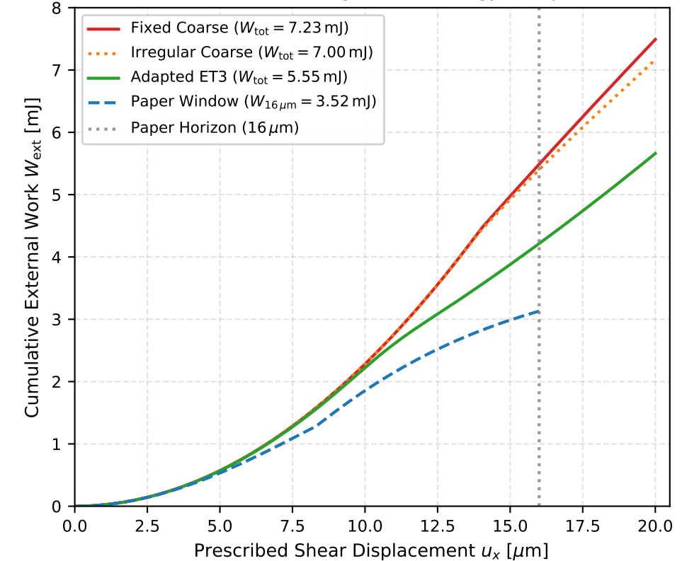
(c) External Work Integration &amp; Energy Dissipation
