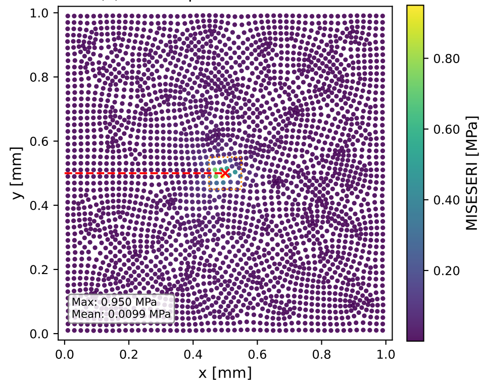
(c) End Step 1: u = 0.0050 mm
