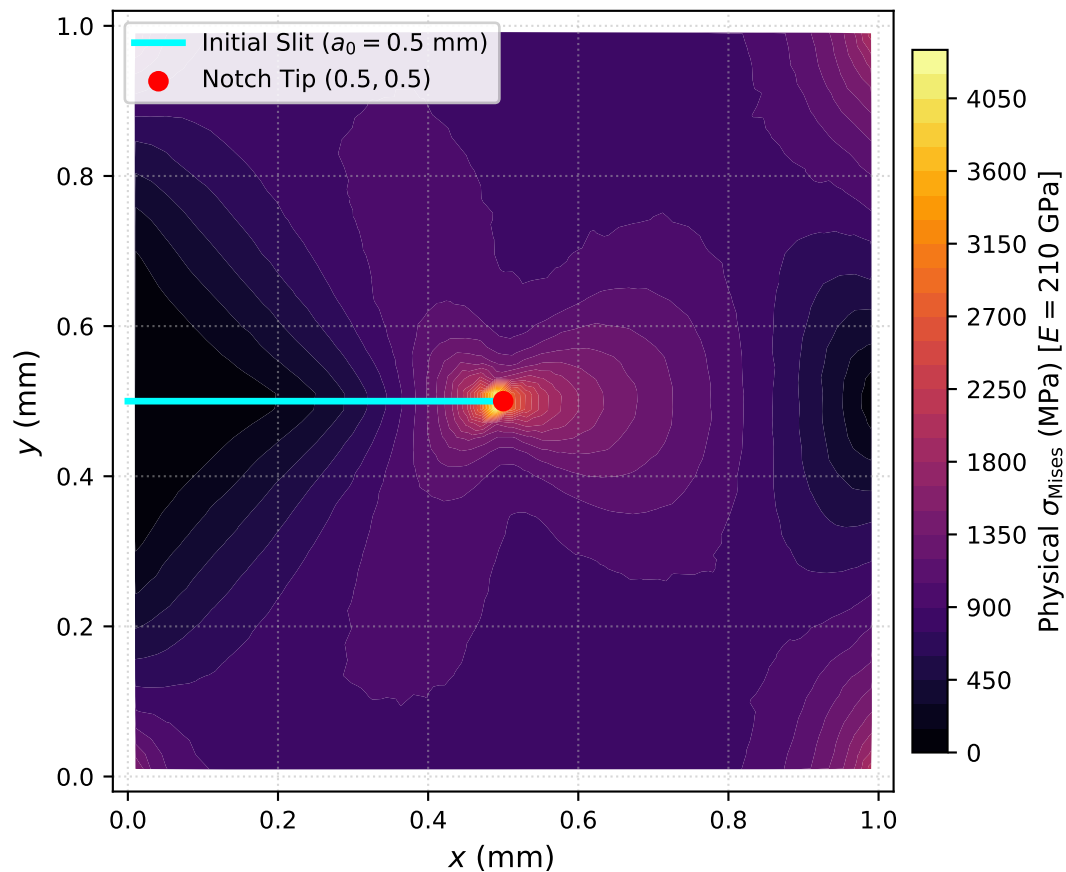
(a) Reconstructed Physical Continuum Stress Field u_x = 10 \mu\text{m} (Step 1 Inc 2000)
