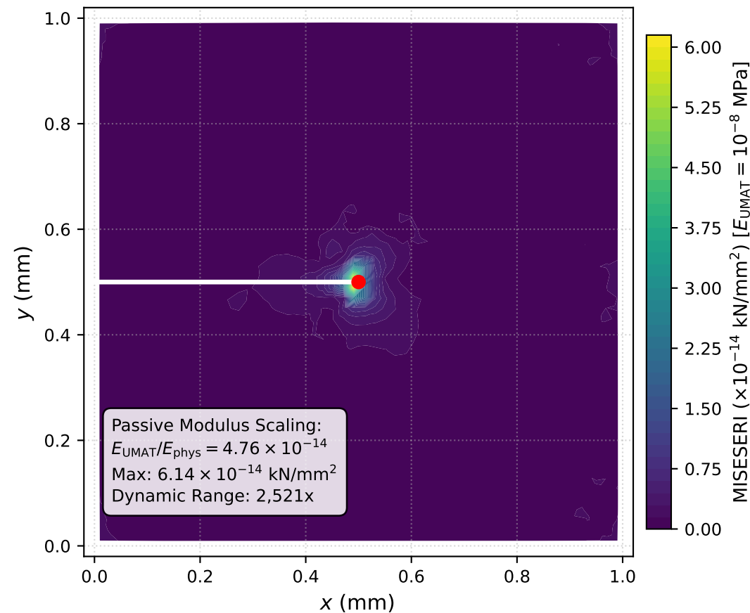
(b) Layer 3 Raw MISESeri Error Indicator Field Abaqus Stress Recovery Error ( 10^{-14} Order Verified)
