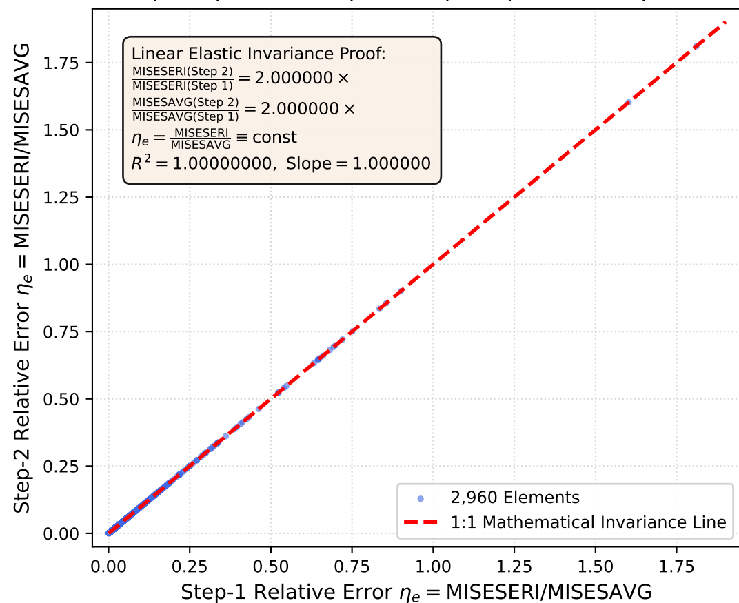
(c) Relative Error Indicator Scale-Invariance \eta_e(\text{Step 1}, u_x = 10 \mu\text{m}) vs \eta_e(\text{Step 2}, u_x = 20 \mu\text{m})
