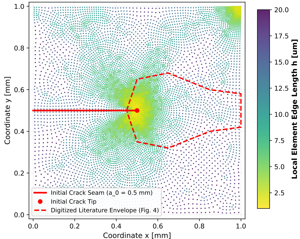
(b) Diagnostic 2.0% Target (11,737 Elements) Localized Crack-Tip Refinement Corridor
