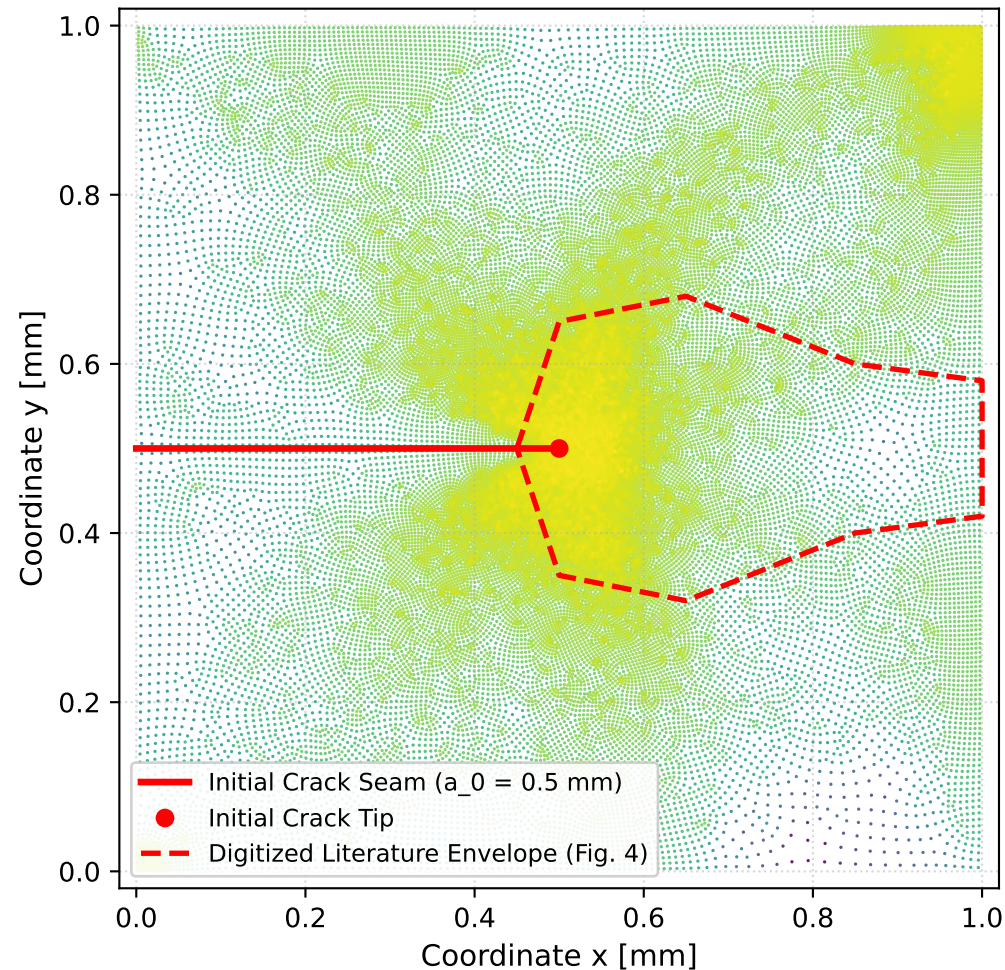
(a) Project 1.0% Target (48,329 Elements) Global Error Percolation over Entire Plate
