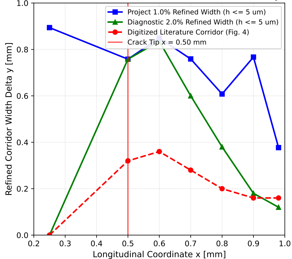
(b) Transverse Refinement Corridor Width \Delta y(x)
