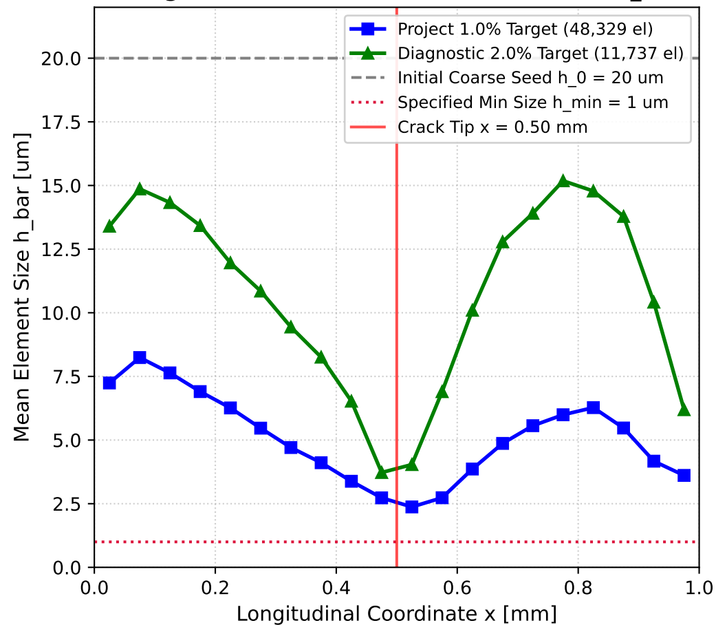
(a) Longitudinal Mean Element Size Profile \bar{h}(x)
