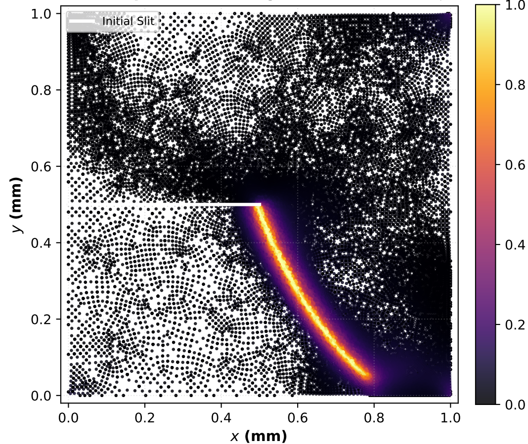
(a) Full Specimen Damage Field at u_x = 19.1\mu\text{m}
