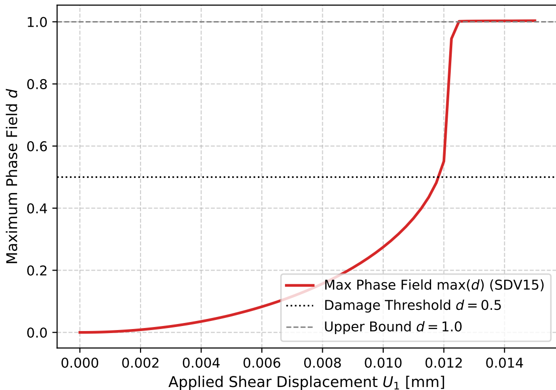
Mode-II Phase-Field Evolution (u015, Job 1379481.mm.master02)
