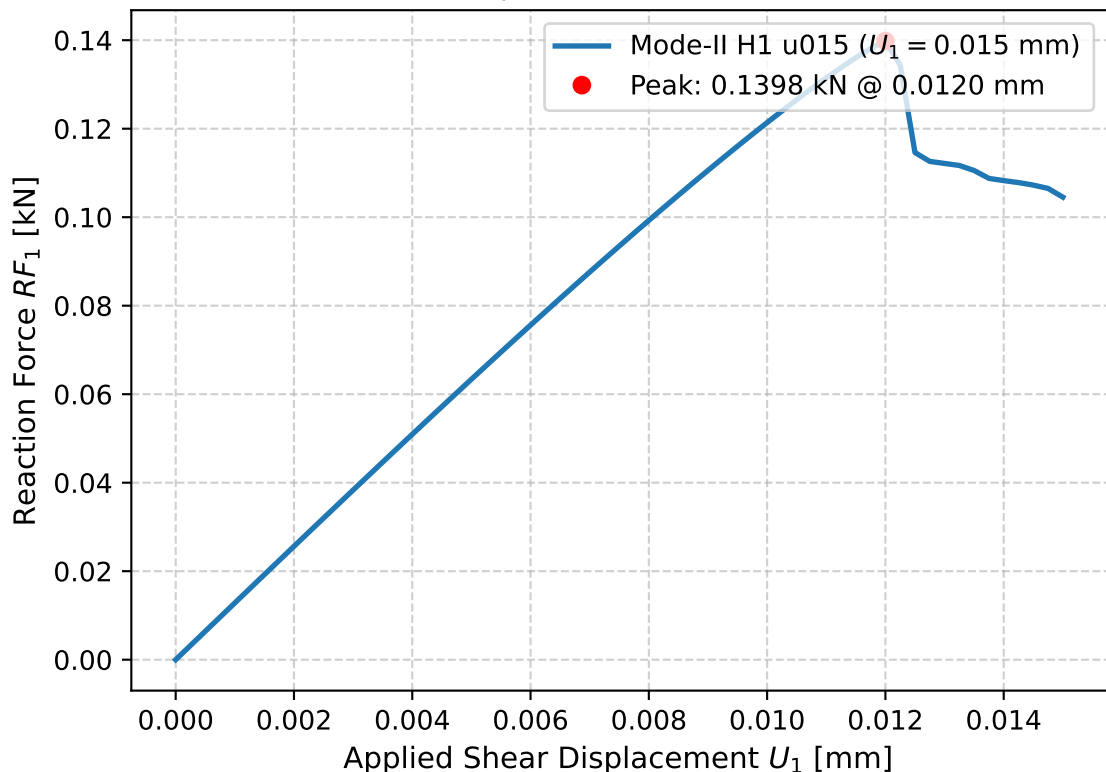
Mode-II Pure Shear Response (u015, Job 1379481.mm.master02)
