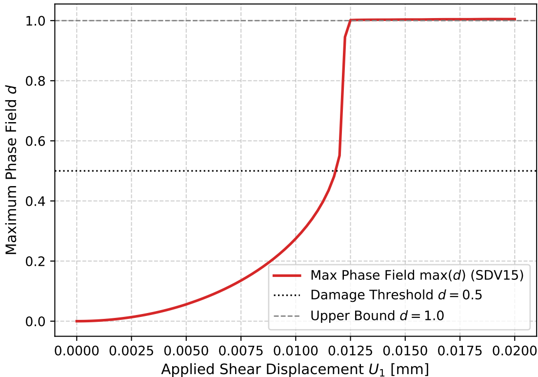
Mode-II Phase-Field Evolution (u020, Job 1379482.mmaster02)
