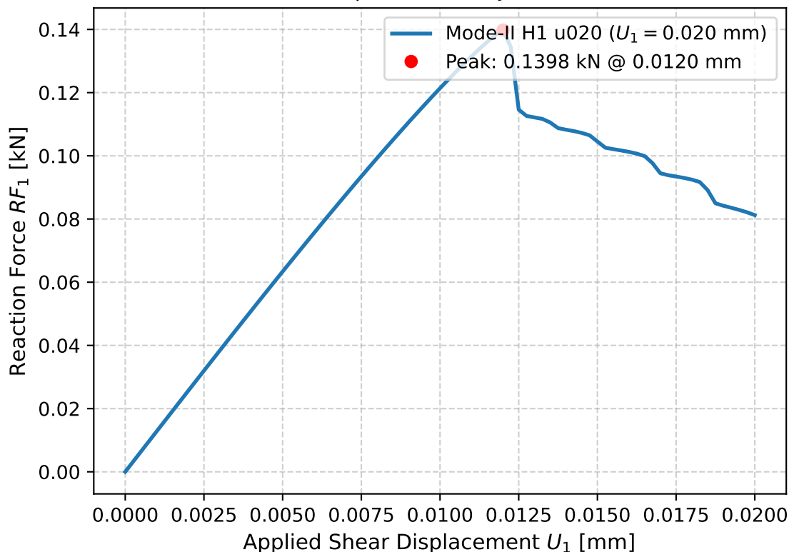
Mode-II Pure Shear Response (u020, Job 1379482.mm.master02)
