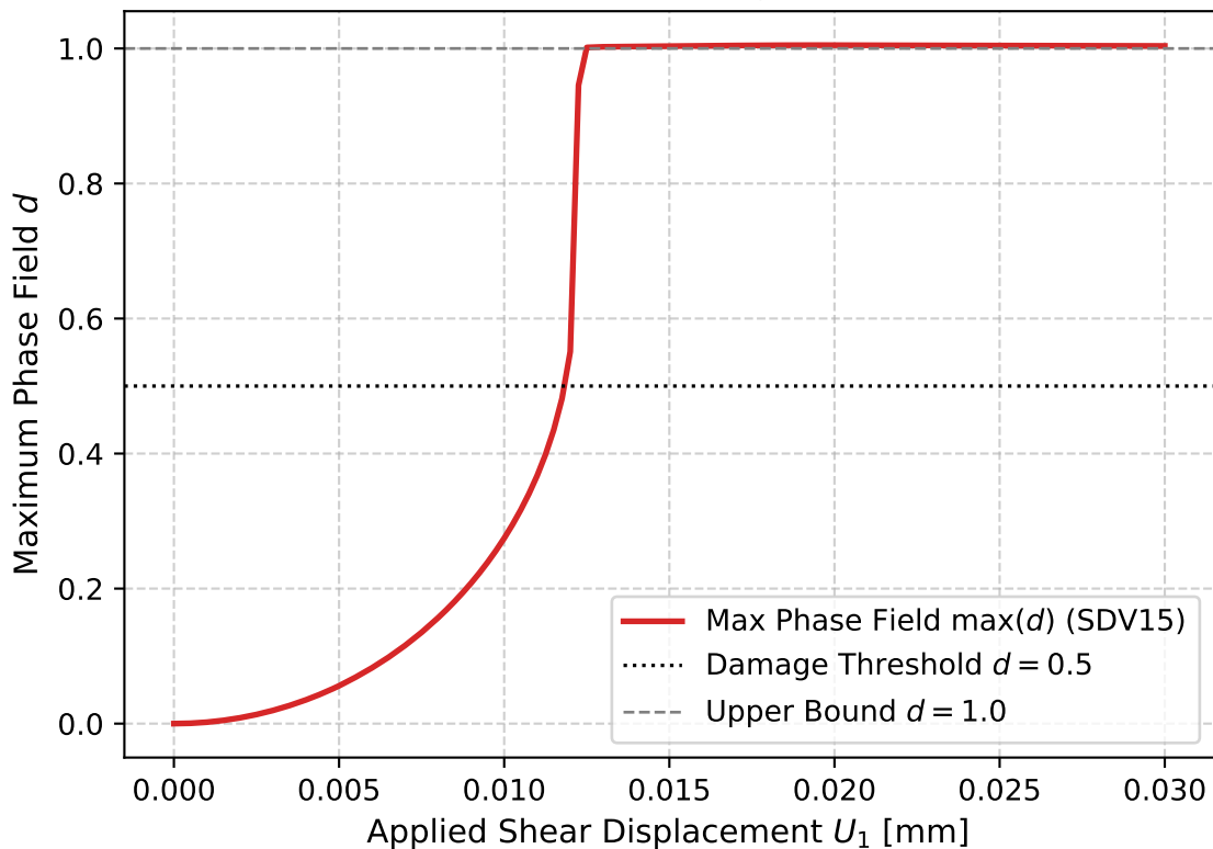
Mode-II Phase-Field Evolution (u030, Job 1379483.mmaster02)
