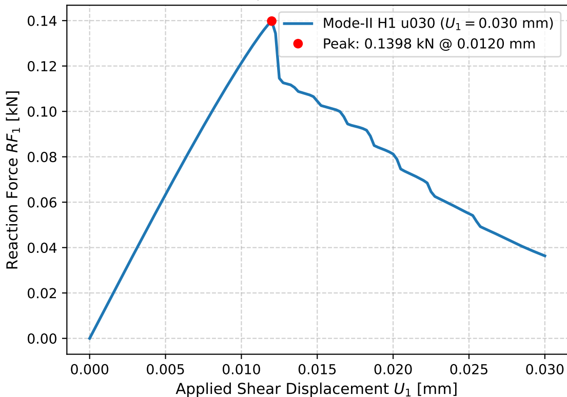
Mode-II Pure Shear Response (u030, Job 1379483.mm.master02)
