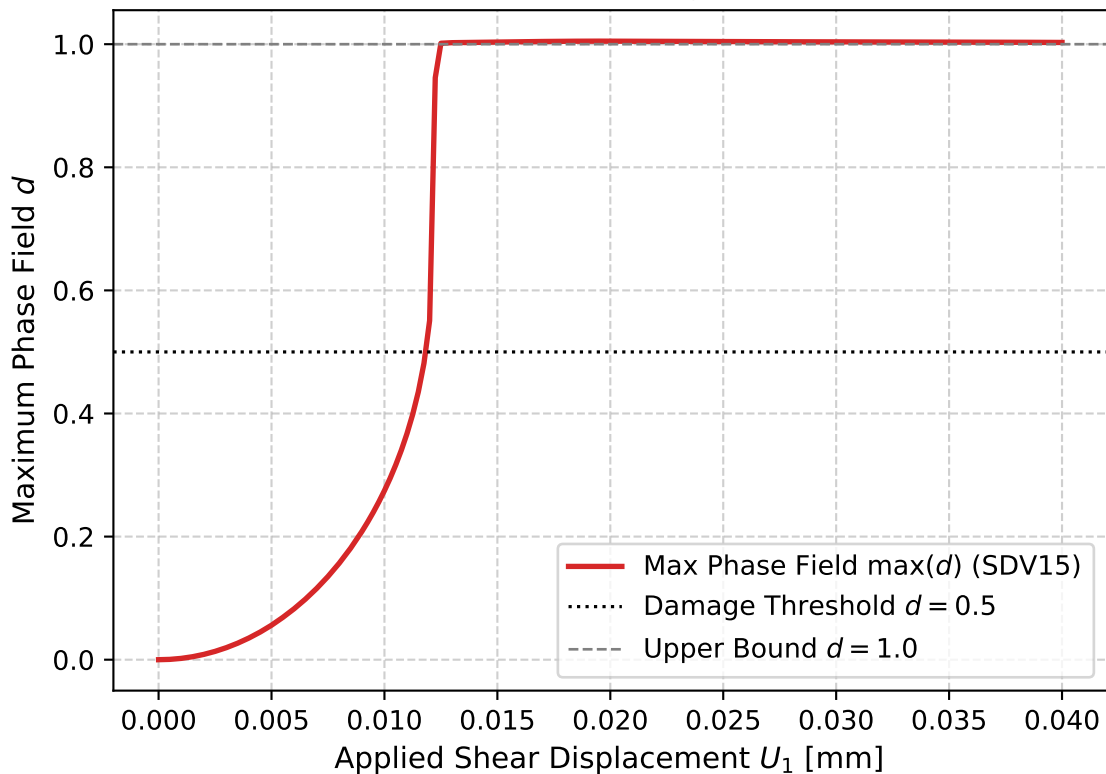
Mode-II Phase-Field Evolution (u040, Job 1379484.mm.master02)
