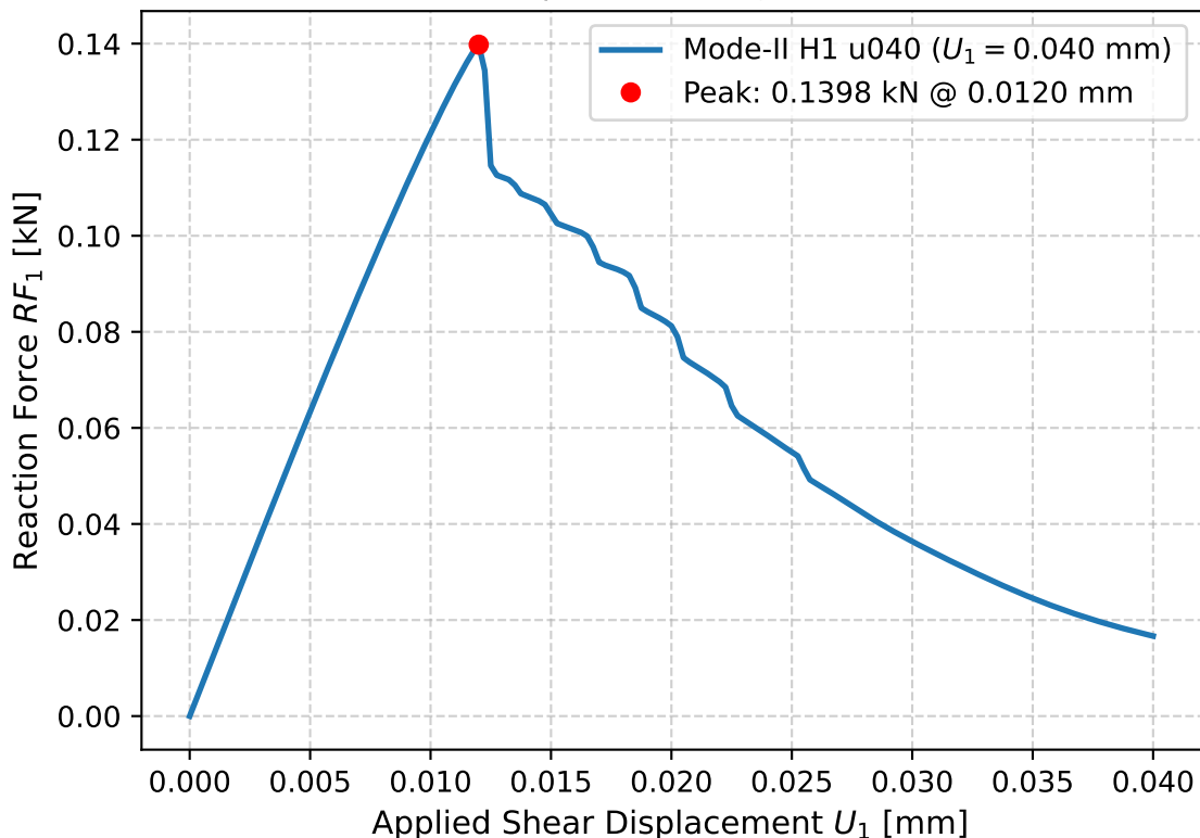
Mode-II Pure Shear Response (u040, Job 1379484.mm.master02)
