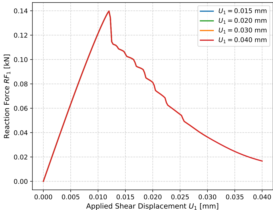
Mode-II H_1 Endpoint Sweep: Force-Displacement
