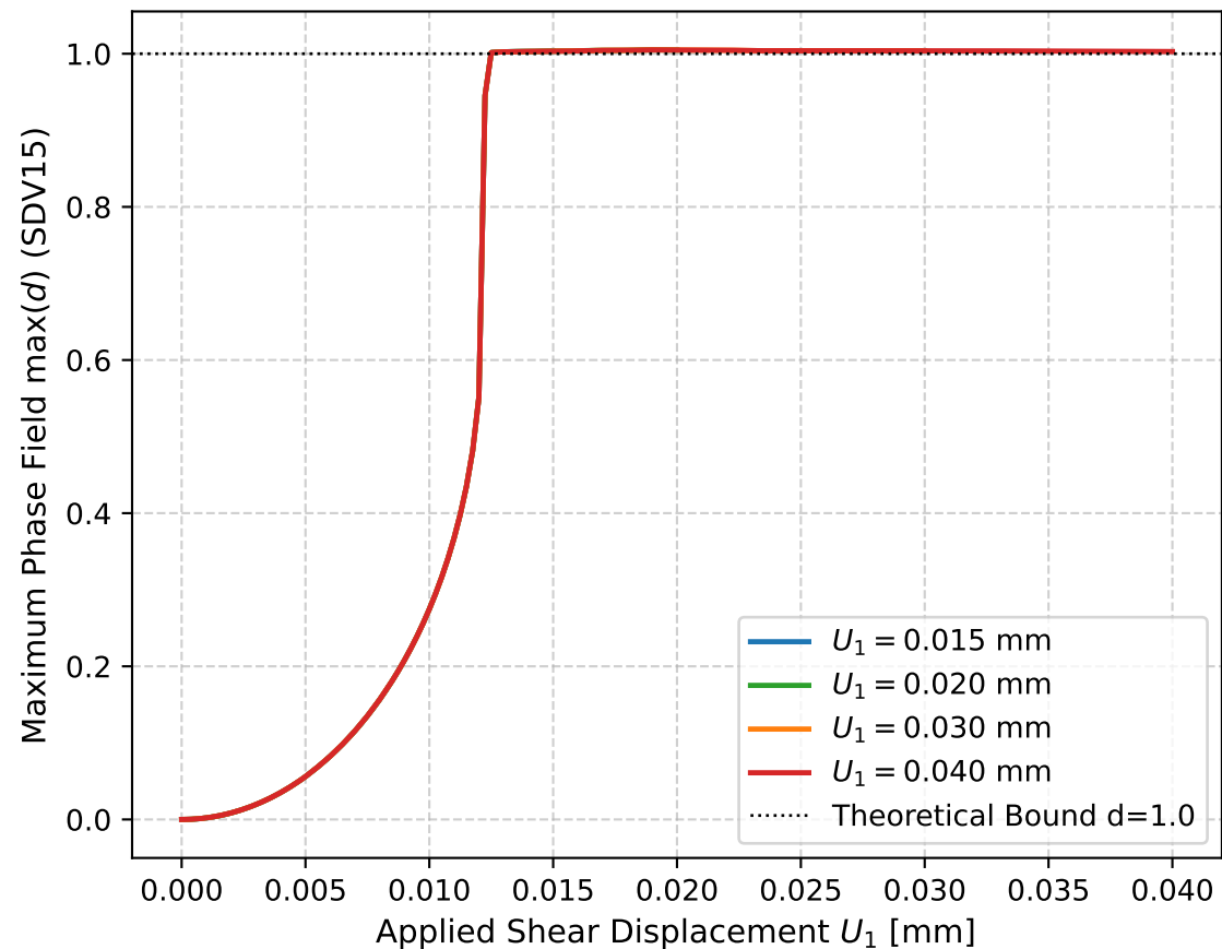
Mode-II H_1 Endpoint Sweep: Damage Evolution
