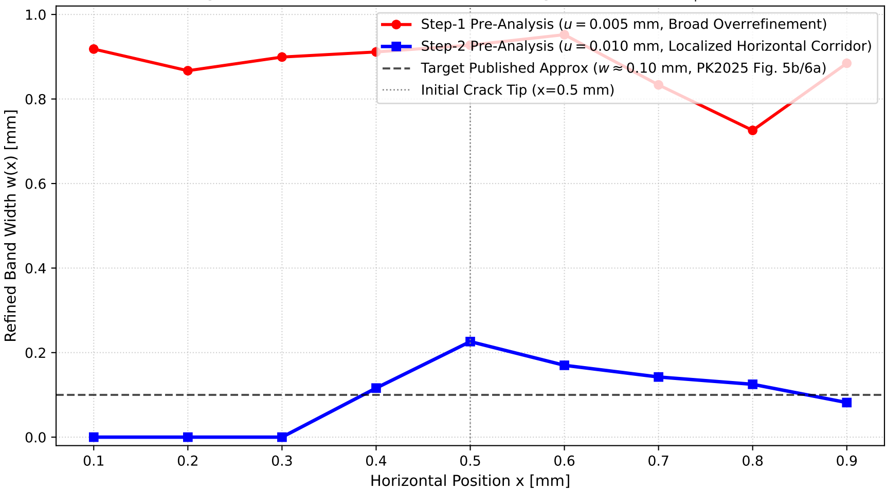
Stage 14: Refined Band Width w(x) along Crack Path ( h_{eq} \leq 5 \mu\text{m} )
