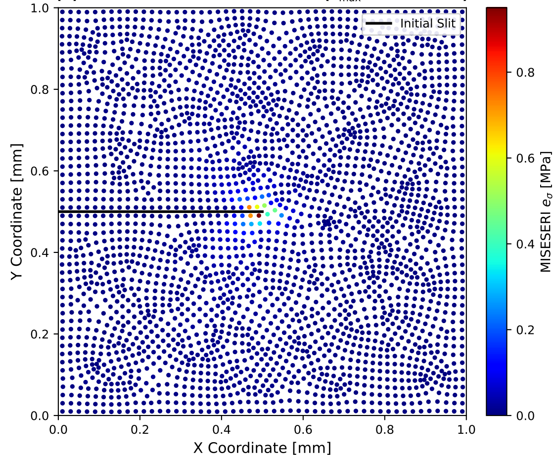
(b) Standard Continuum Control ( e_{\max} = 0.950 MPa)
