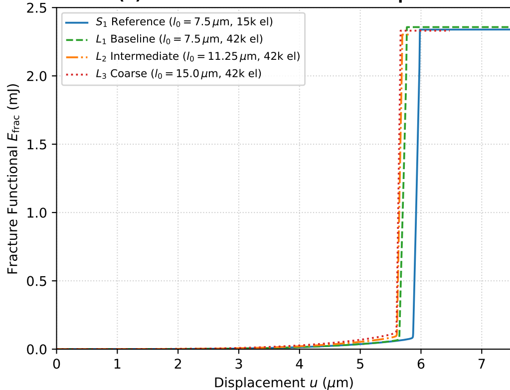
(b) Crack-Surface Functional Dissipation
