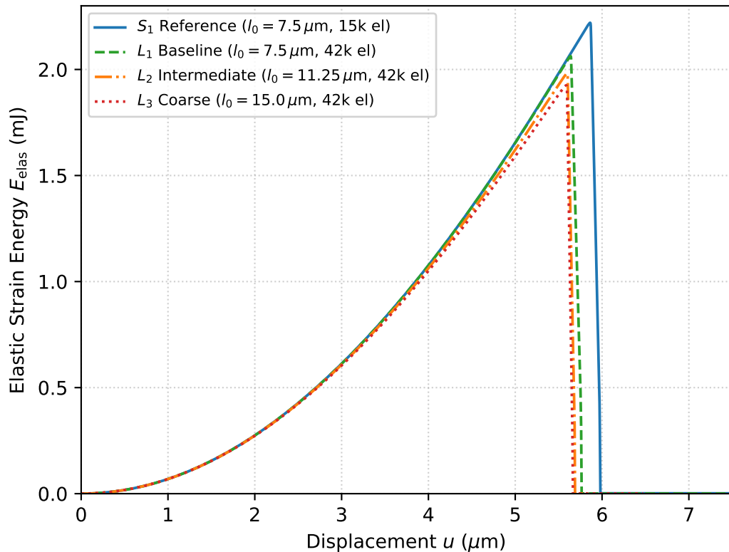
(a) Elastic Strain Energy Storage
