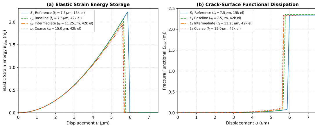
Fig. 4.24.: Energy evolution and partitioning dynamics across phase-field length scales: (a) Elastic strain energy storage E_{\text{elas}}(u) ; (b) Crack-surface functional E_{\text{frac}}(u) . Pre-peak damage energy increases with l_0 due to broader regularization zones, while broken-state functional dissipation converges to \sim 2.30\text{--}2.36 \text{ mJ} .
