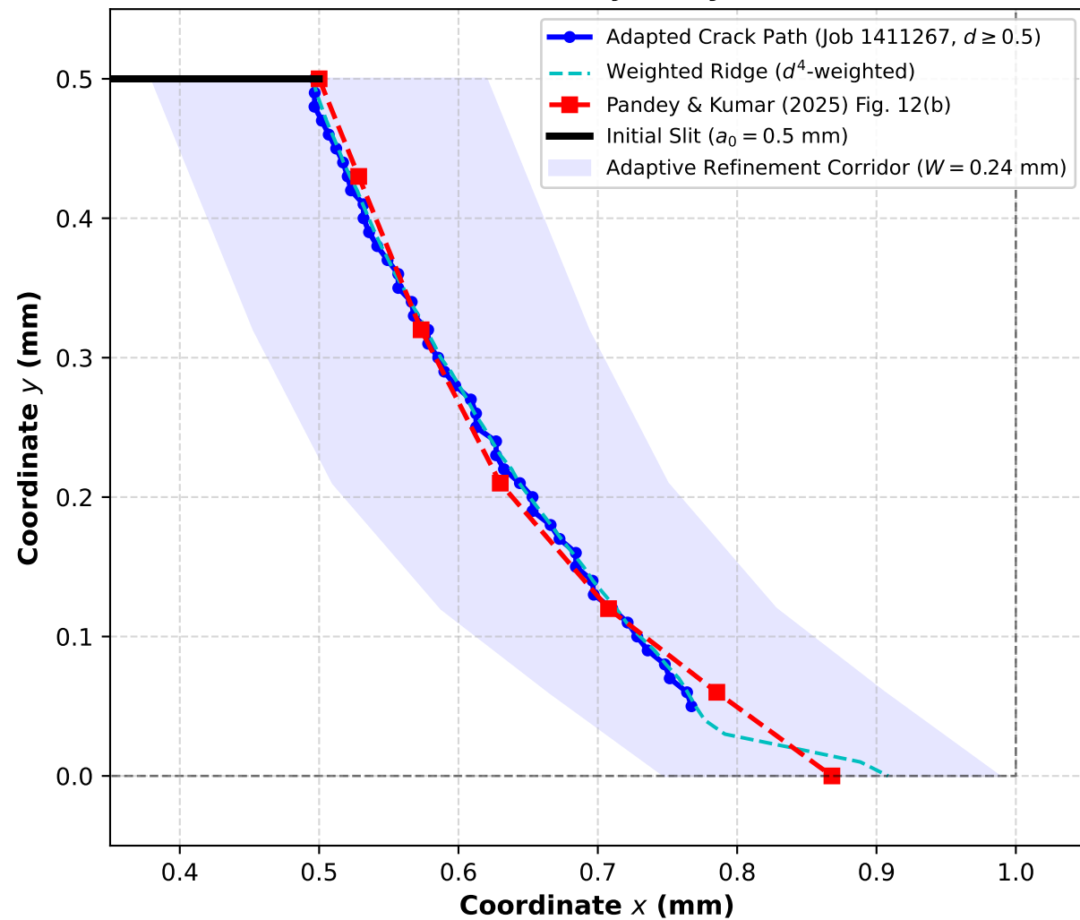
(a) Extracted Crack Trajectory vs. Literature
