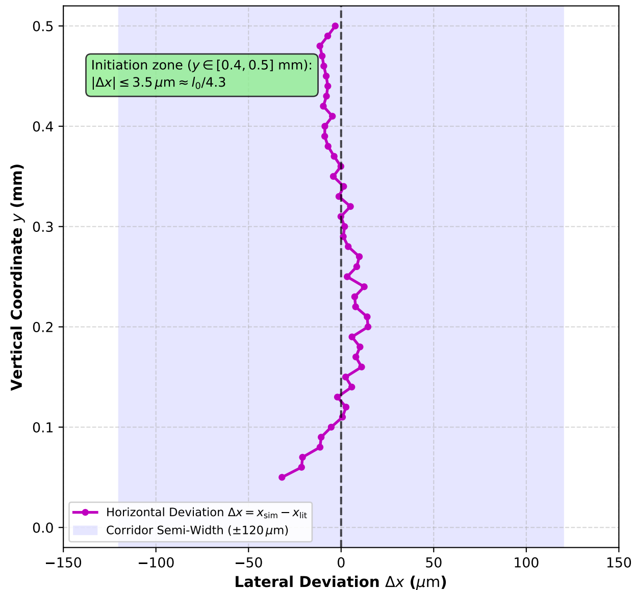
(b) Crack Path Deviation Profile
