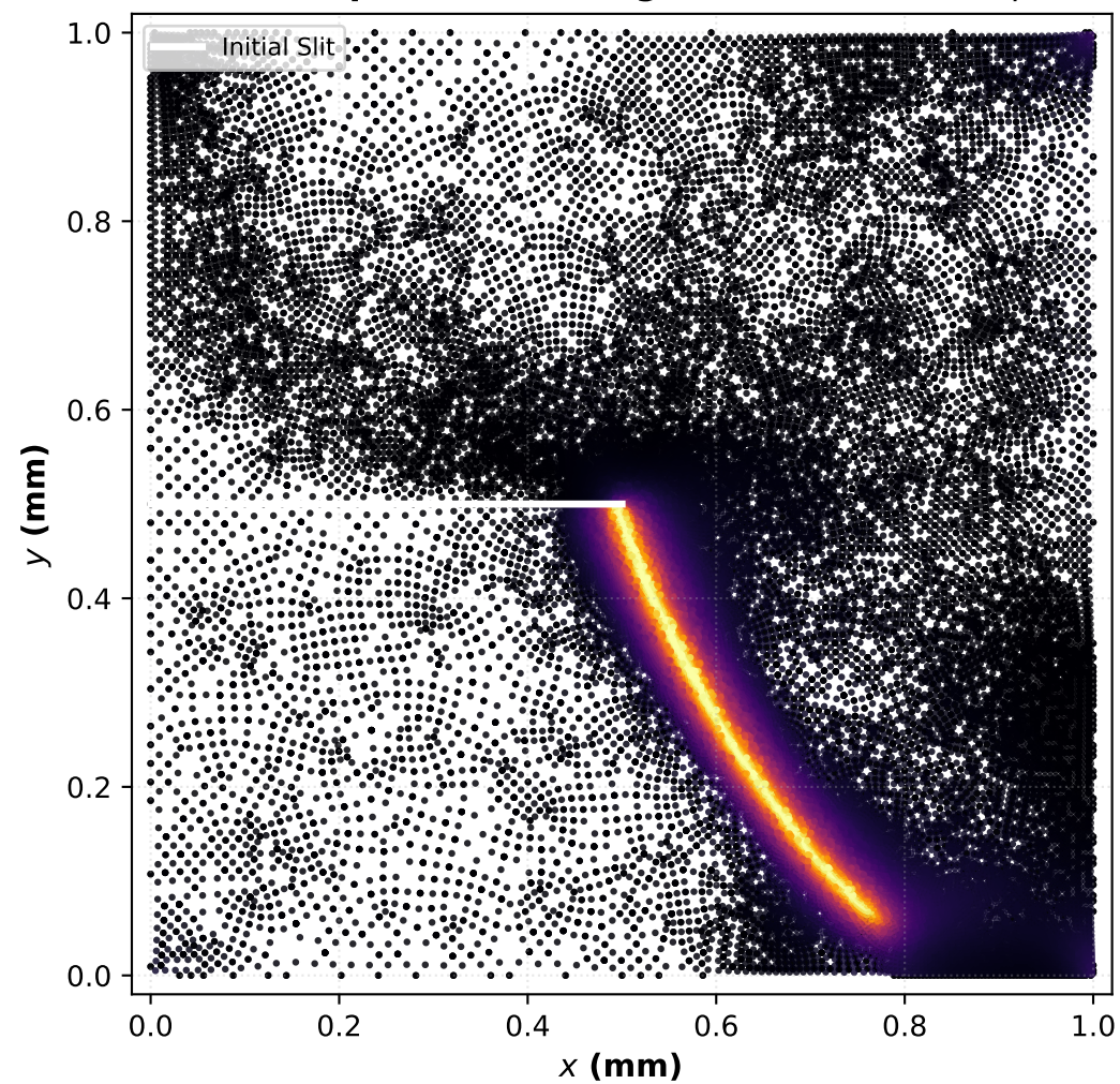
(a) Full Specimen Damage Field at u_x = 18.0\ \mu\text{m}
