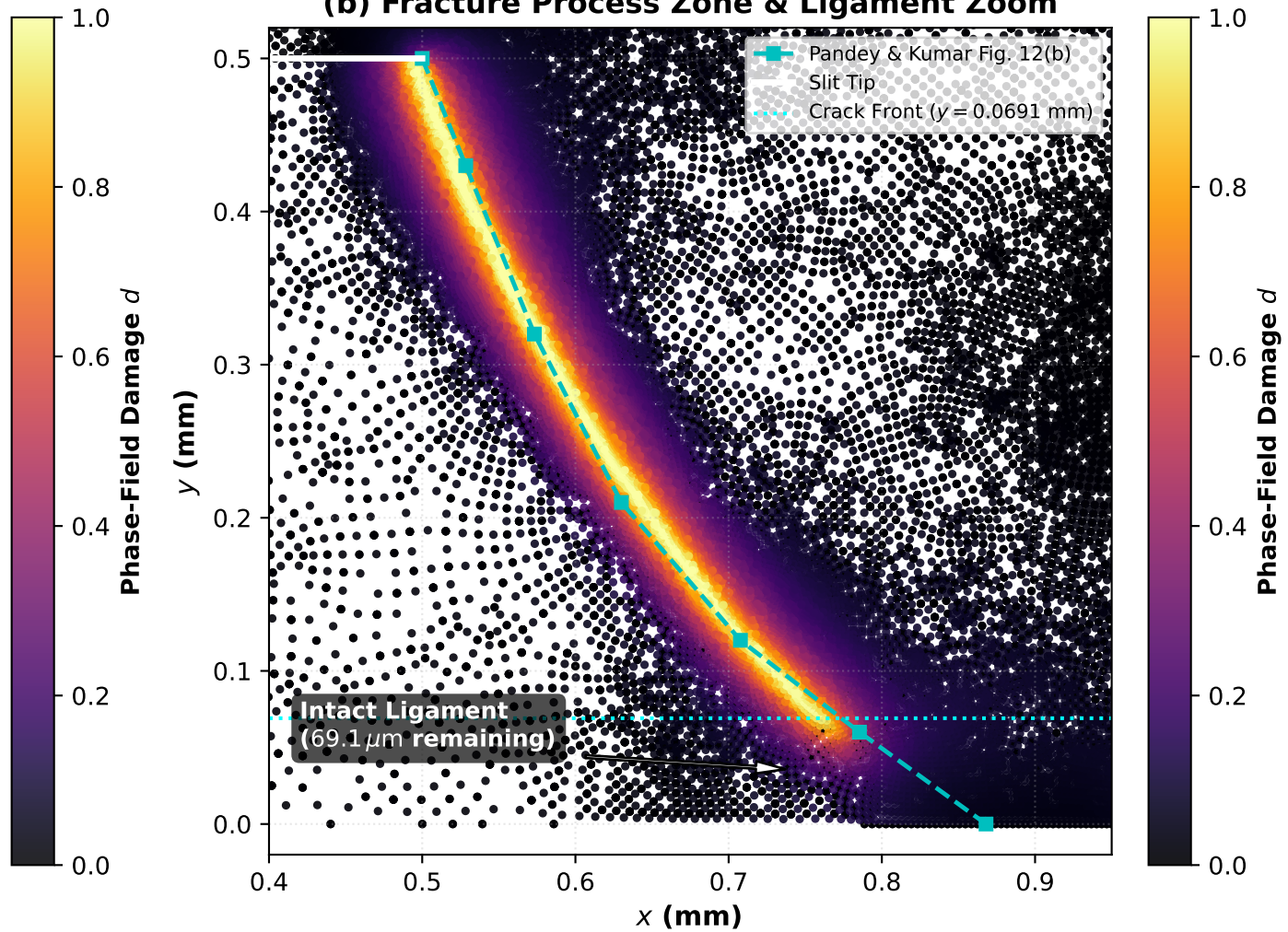
(b) Fracture Process Zone & Ligament Zoom
