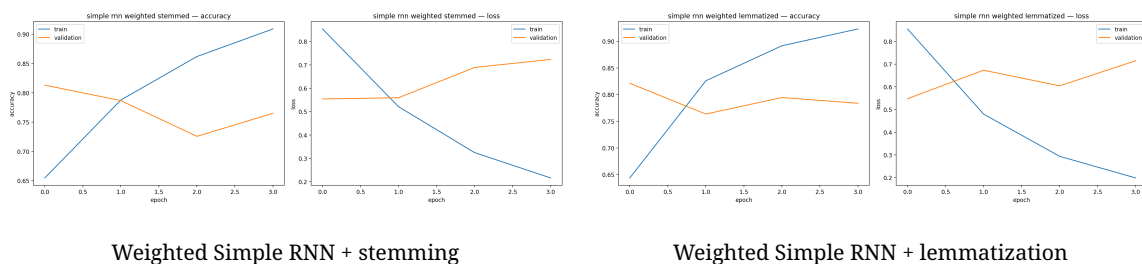
Figure 7: Training curves for class-weighted Simple RNN models.
