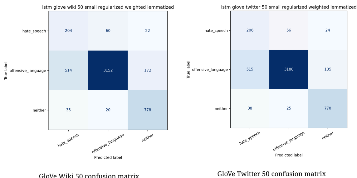
Figure 13: Confusion matrices for pretrained GloVe embedding experiments.
