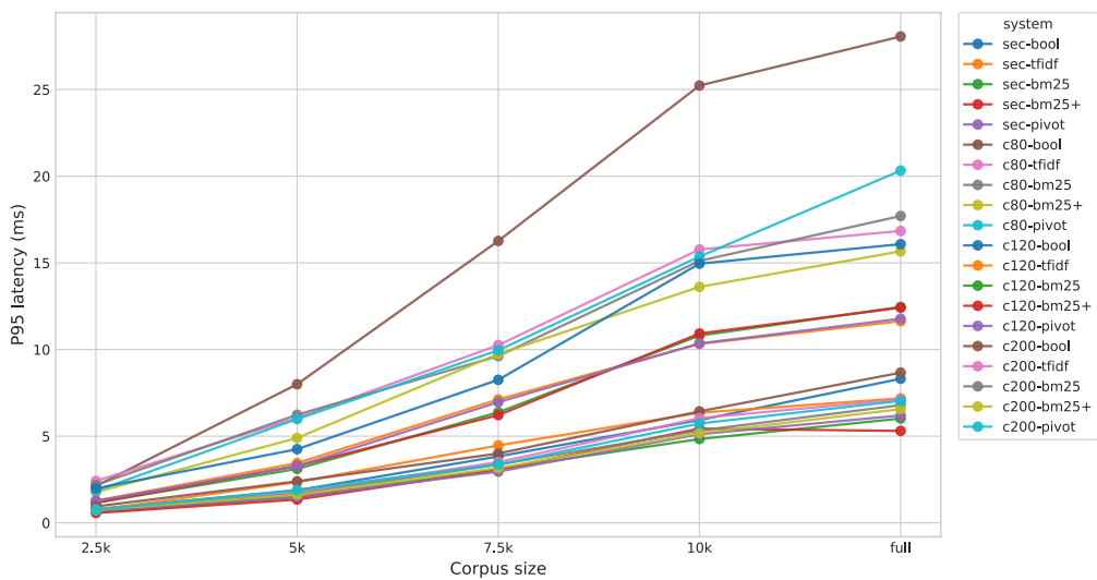
corpus size vs p95 latency
