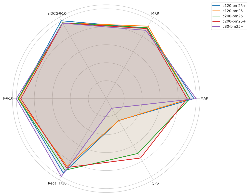
radar chart top systems
