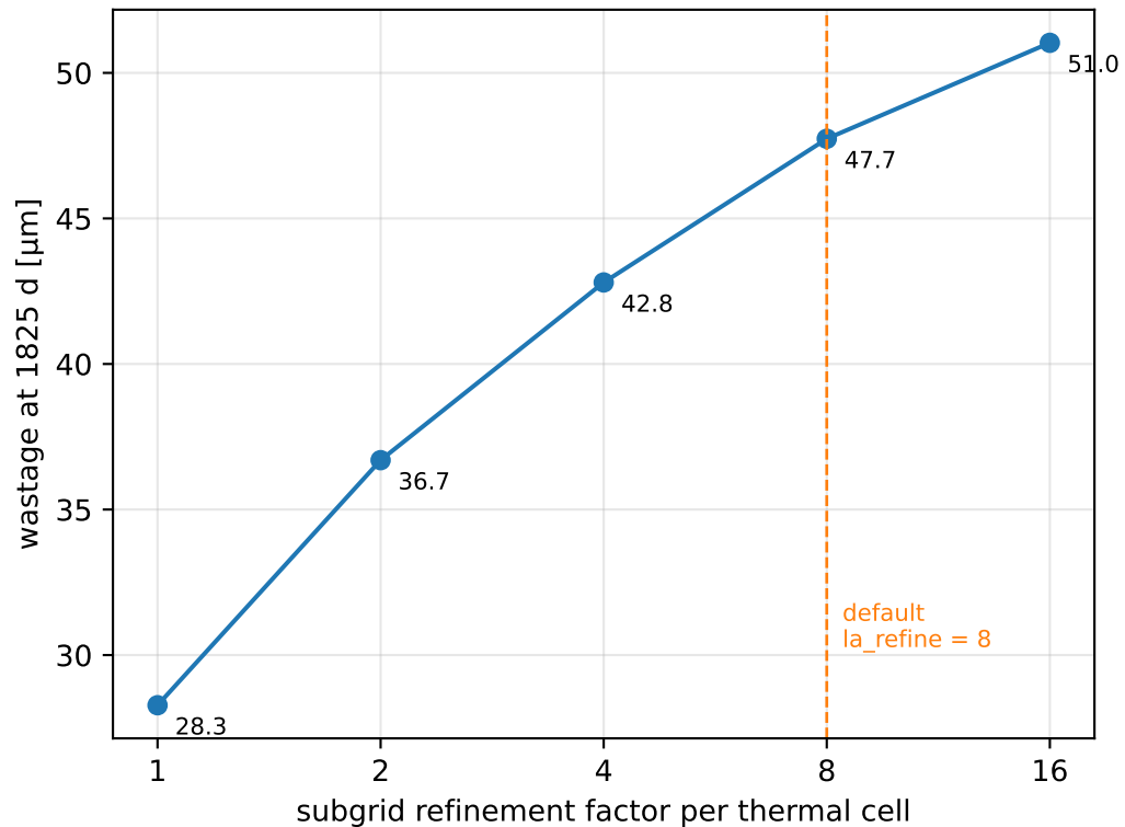
(a) Mesh convergence (IF-AVG, layer 12)
