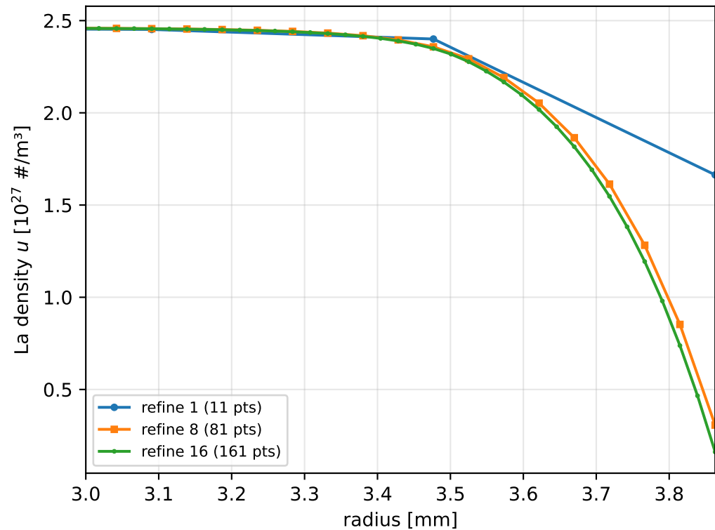
(b) EOL near-interface boundary layer
