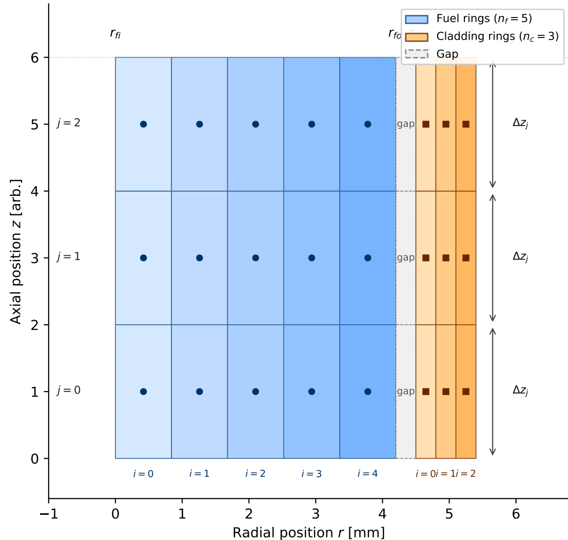
FRED Discretization: n_f fuel rings, n_c cladding rings, n_z axial layers
