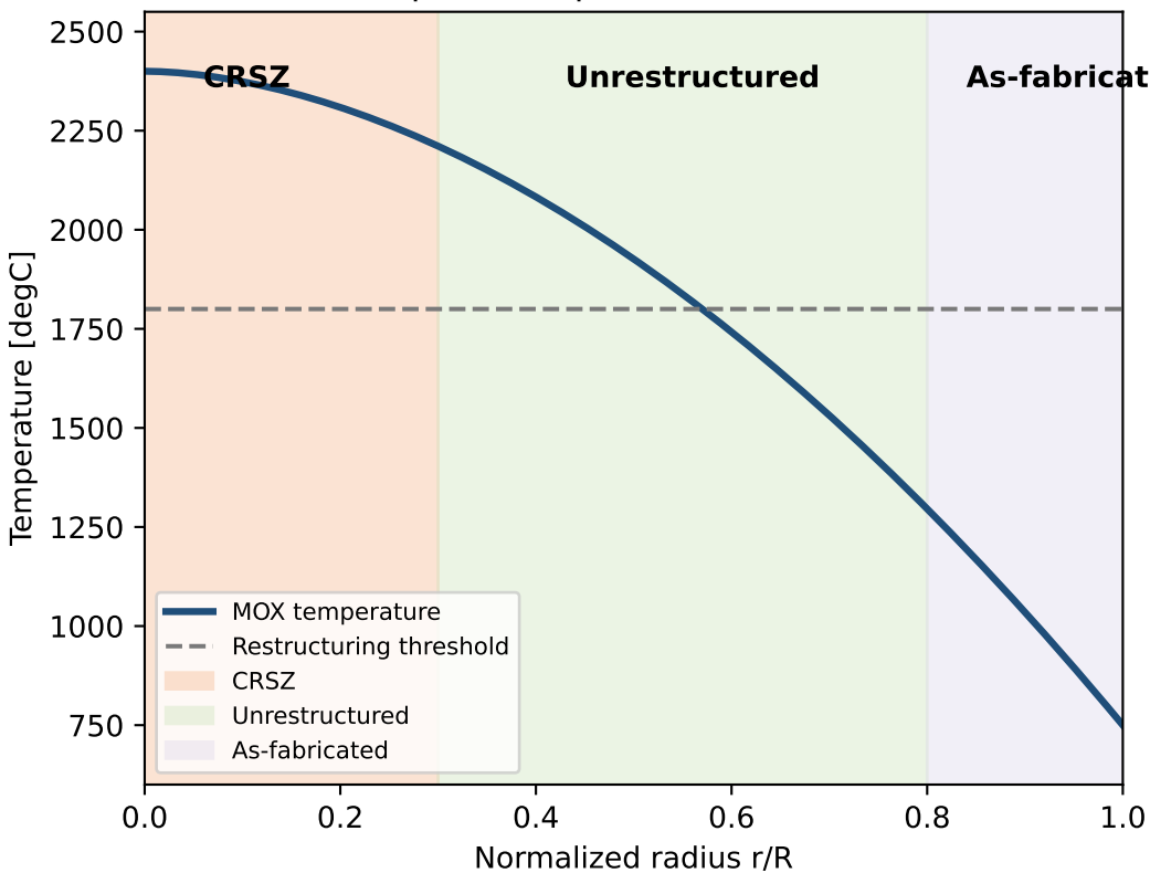
(a) Temperature profile and radial zones
