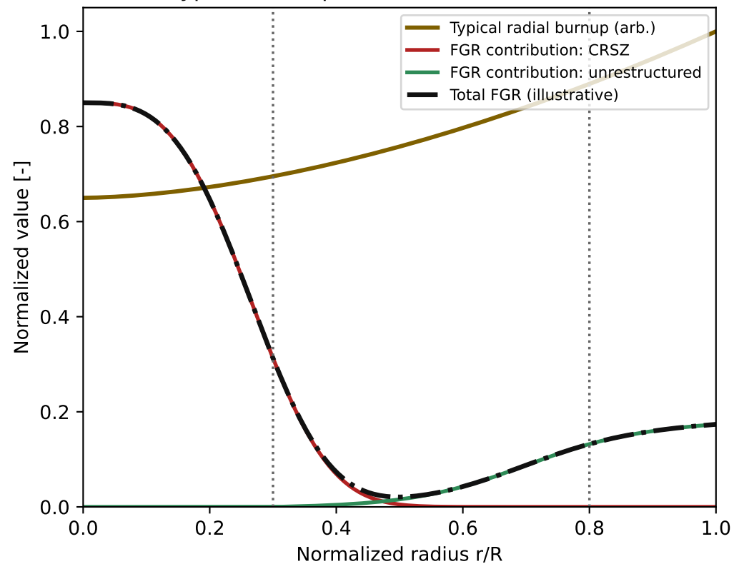
(b) Typical burnup and zone-wise FGR behavior
