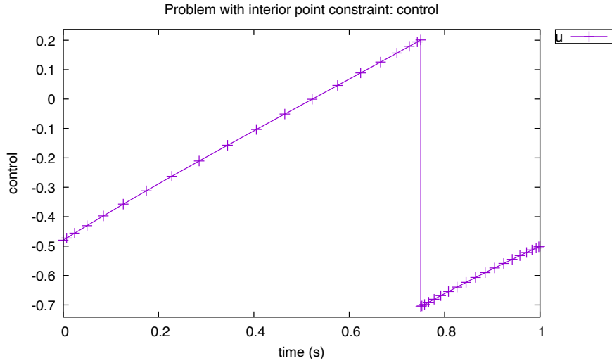
Figure 9: Control for the interior point constraint problem. The jump at t = 0.75 is the phase boundary
