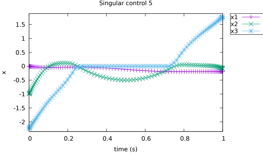
Figure 10: States for the singular control problem
