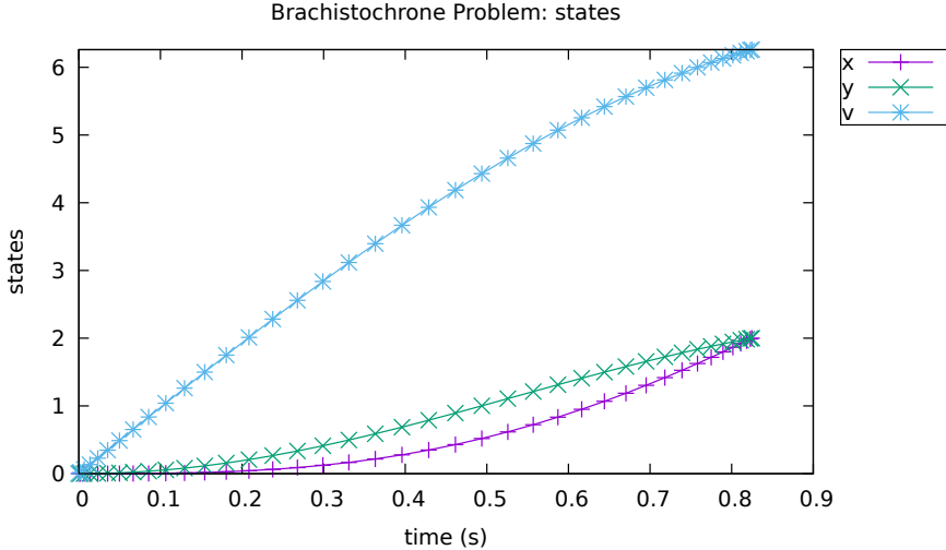
Figure 1: States for the brachistochrone problem
